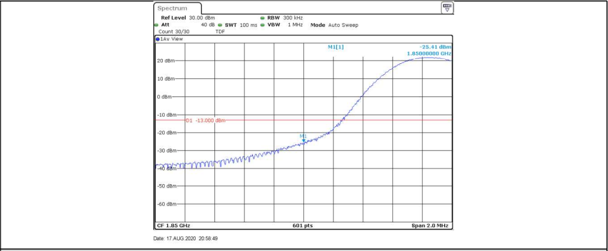
Band2-15MHz-QPSK-18675-75RB#0
