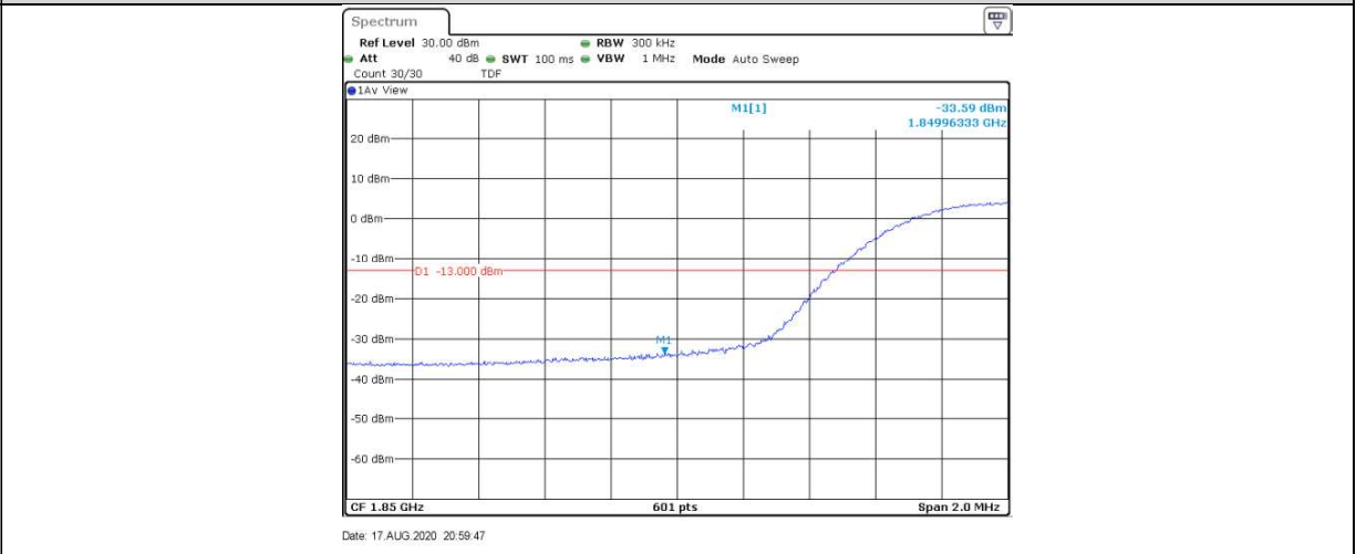
Band2-15MHz-16QAM-19125-1RB#0
