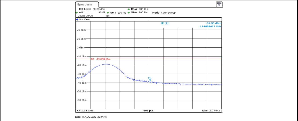
Band2-10MHz-QPSK-19150-1RB#49
