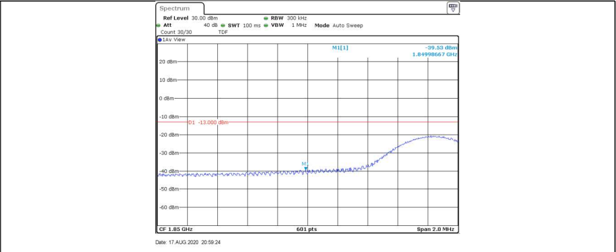
Band2-15MHz-16QAM-18675-75RB#0
