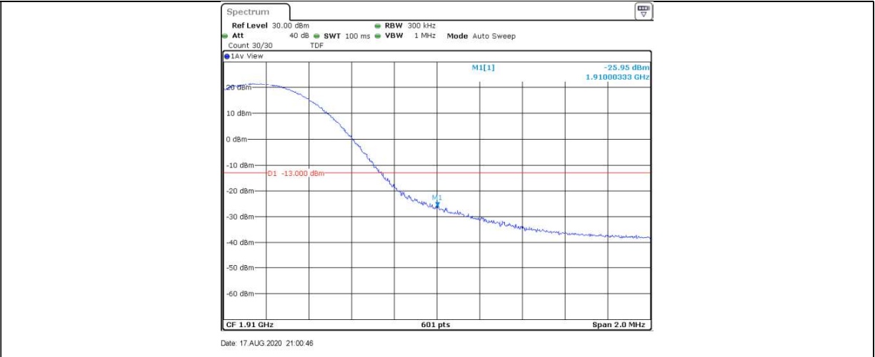
Band2-15MHz-16QAM-19125-75RB#0
