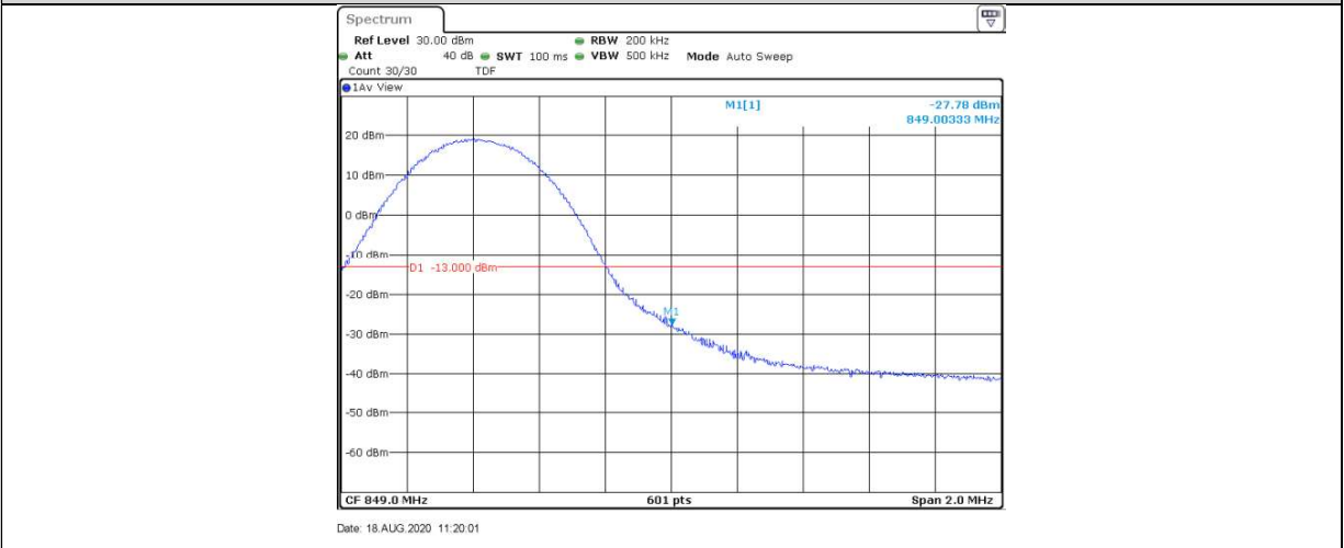
Band5-10MHz-16QAM-20600-50RB#0
