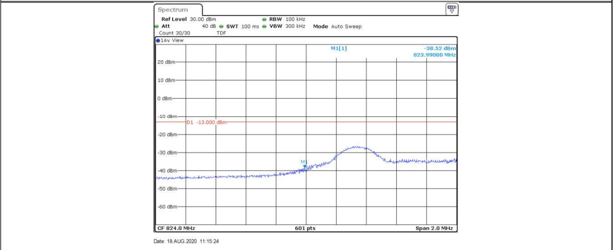
Band5-5MHz-16QAM-20425-1RB#0
