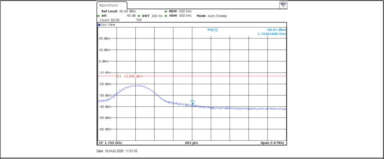
Band4-10MHz-QPSK-20350-50RB#0
