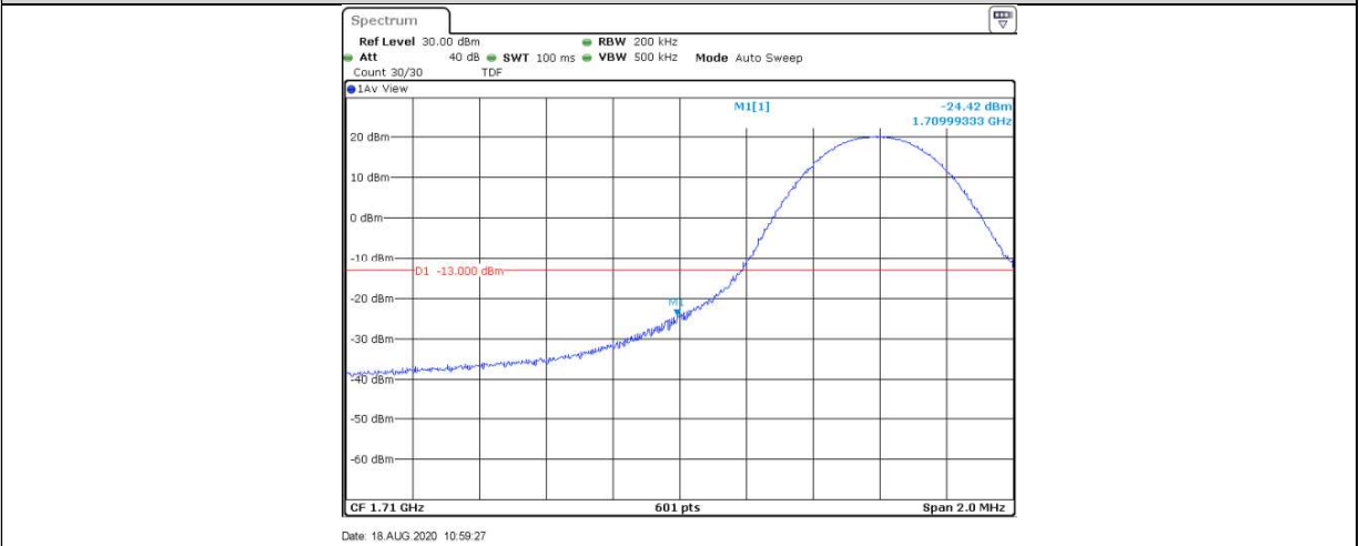
Band4-10MHz-QPSK-20000-1RB#49
