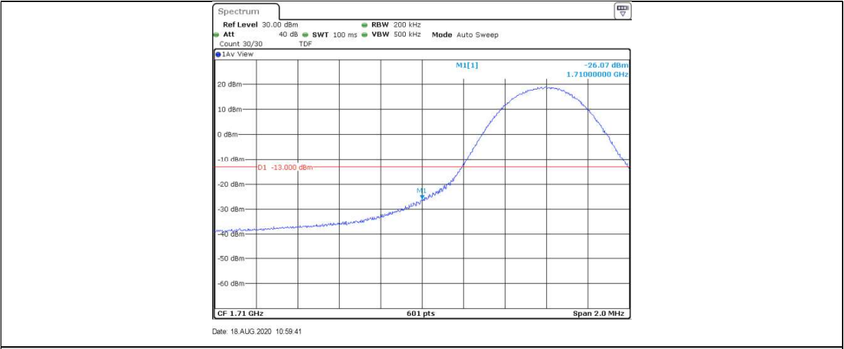
Band4-10MHz-16QAM-20000-50RB#0
