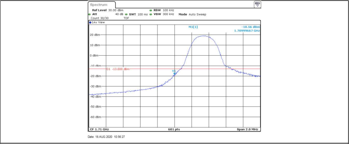
Band4-5MHz-QPSK-19975-25RB#0
