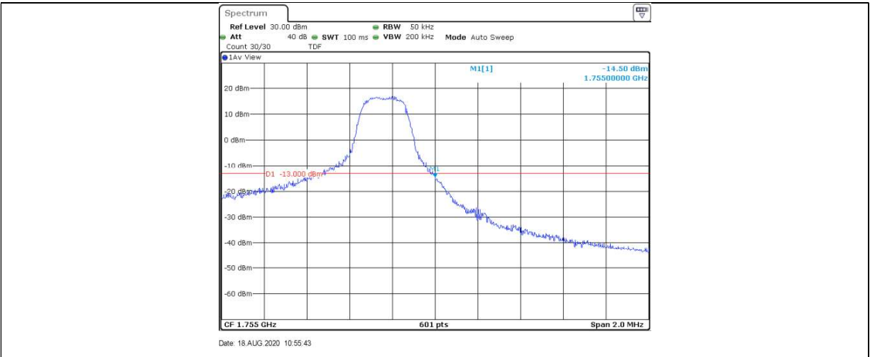
Band4-3MHz-16QAM-20385-15RB#0
