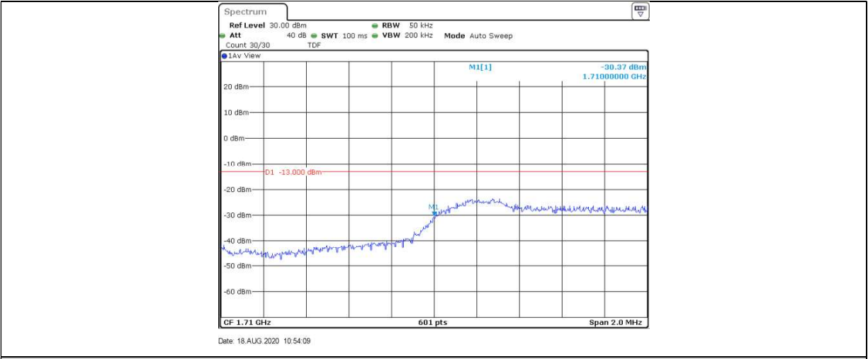
Band4-3MHz-16QAM-19965-15RB#0
