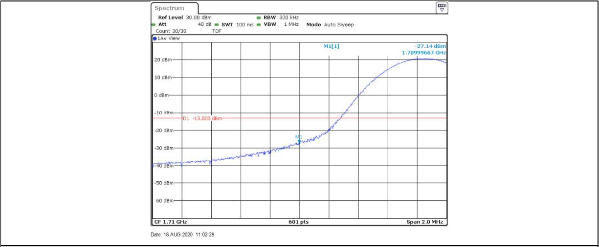
Band4-15MHz-QPSK-20025-75RB#0
