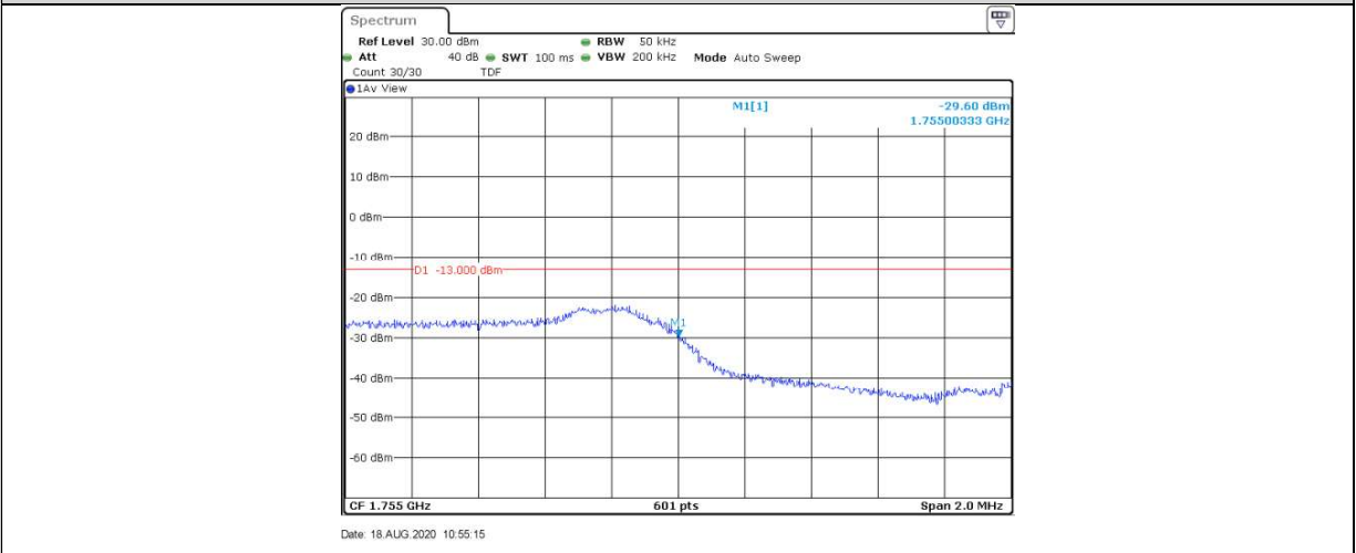
Band4-3MHz-16QAM-20385-1RB#14
