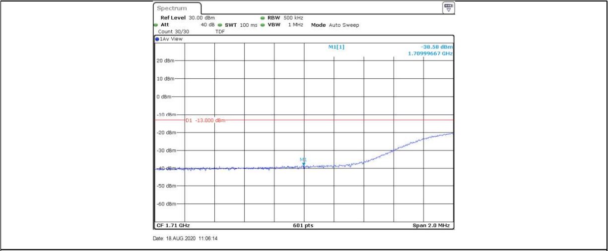
Band4-20MHz-16QAM-20050-100RB#0
