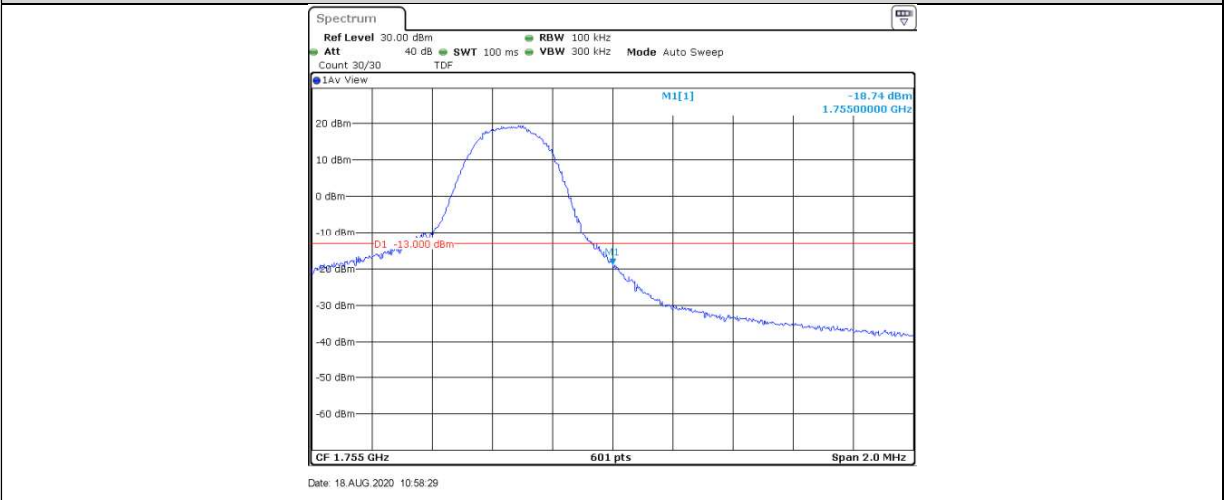
Band4-5MHz-QPSK-20375-1RB#0
