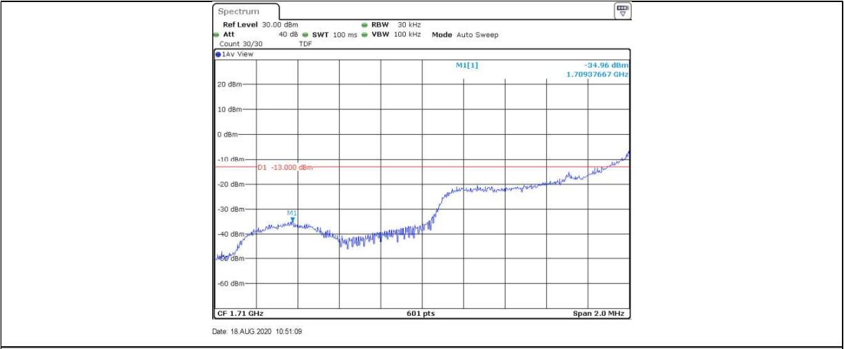
Band4-1.4MHz-16QAM-19957-6RB#0
