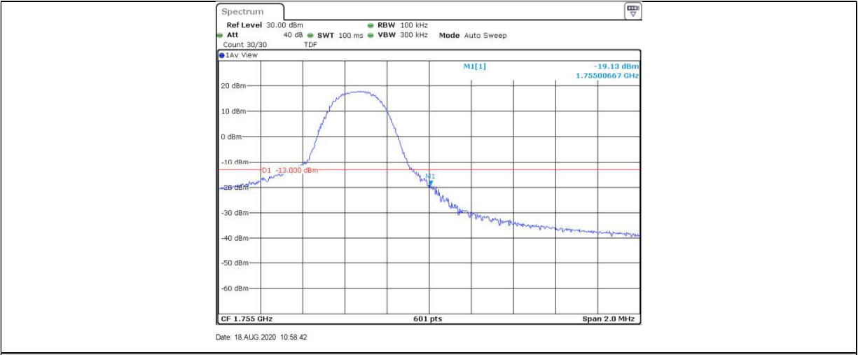
Band4-5MHz-16QAM-20375-25RB#0
