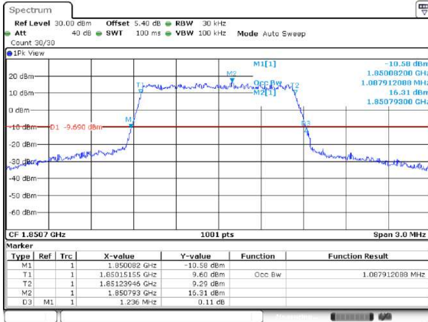
Band25-1.4MHz-QPSK-26047-6RB#0-1.088
