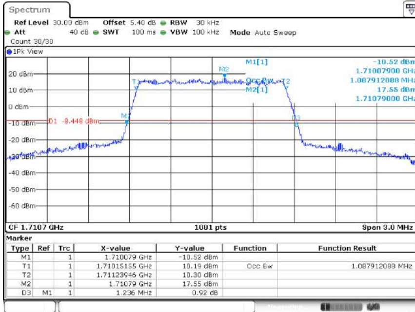
Band4-1.4MHz-QPSK-19957-6RB#0-1.088
