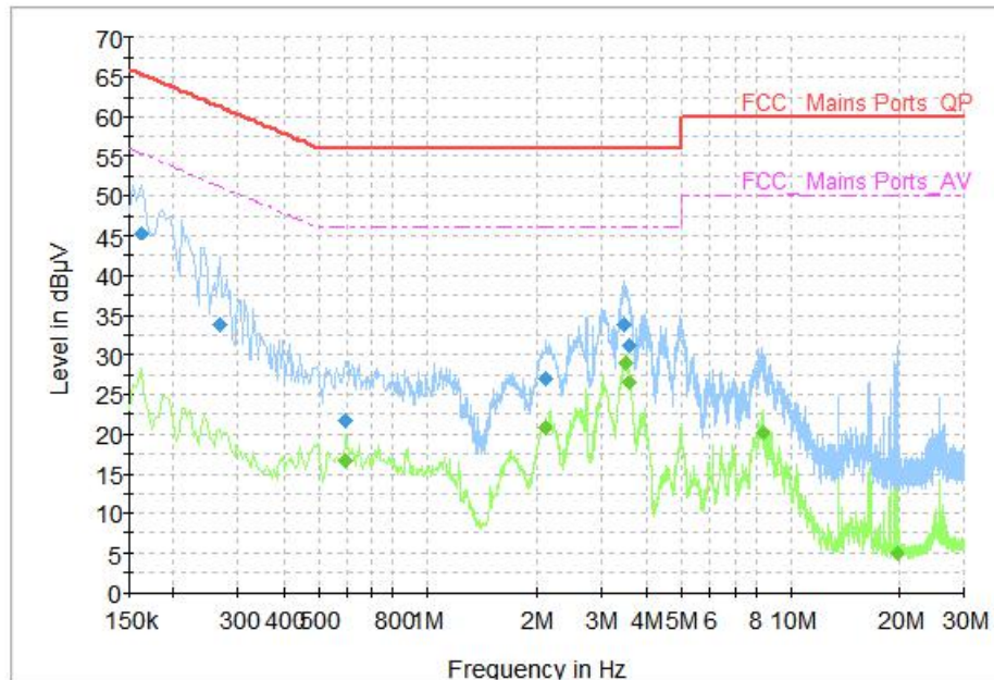
Figure A.3 Conducted Emission
