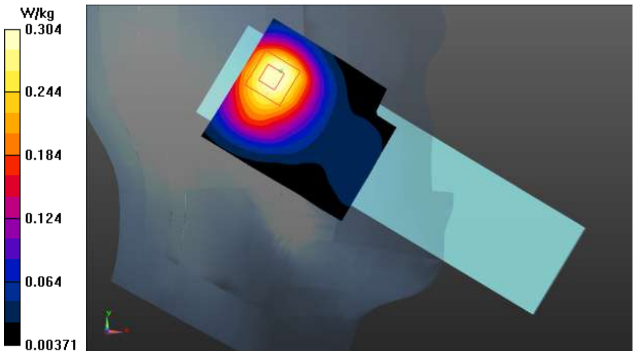
Fig.13 WCDMA Band 4
