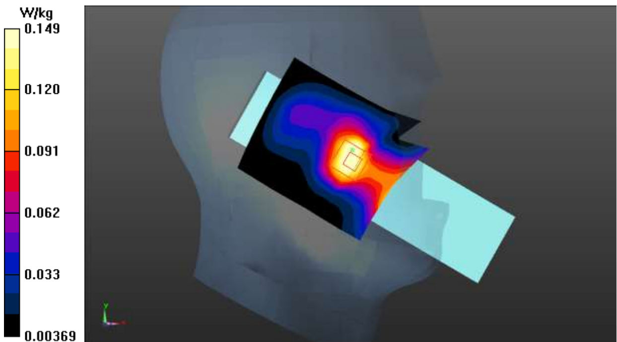
Fig.11 WCDMA Band 2
