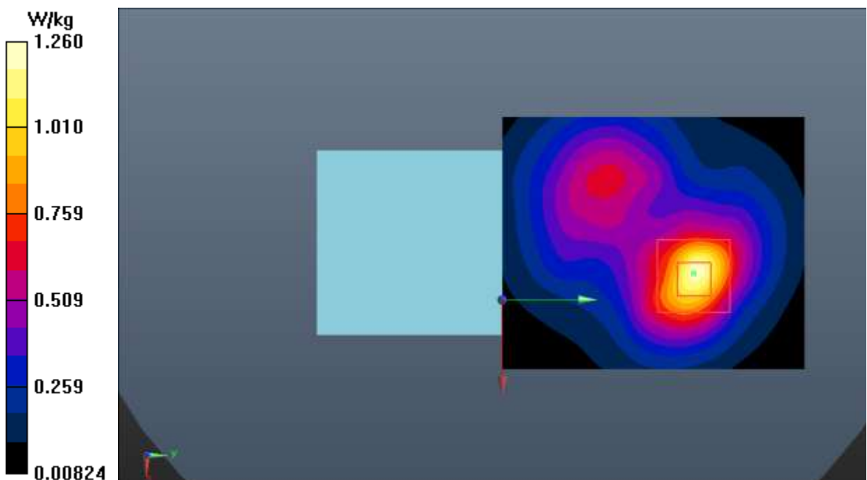
Fig.28 LTE Band 41
