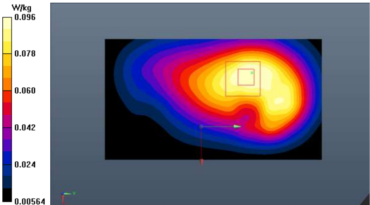
Fig.22 LTE Band 13
