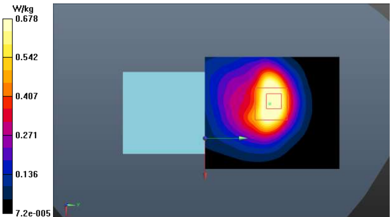
Fig.4 GSM 1900
