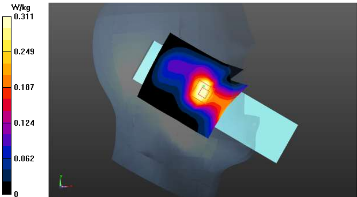
Fig.23 LTE Band 25
