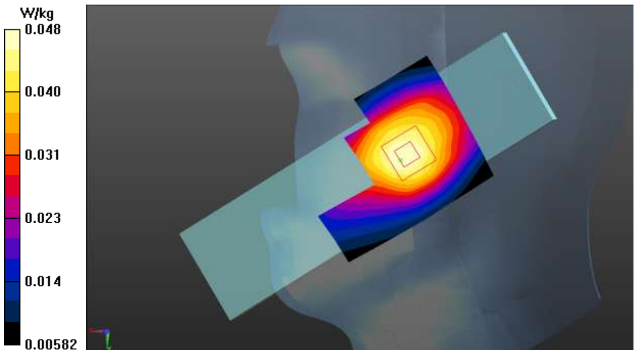
Fig.21 LTE Band 13
