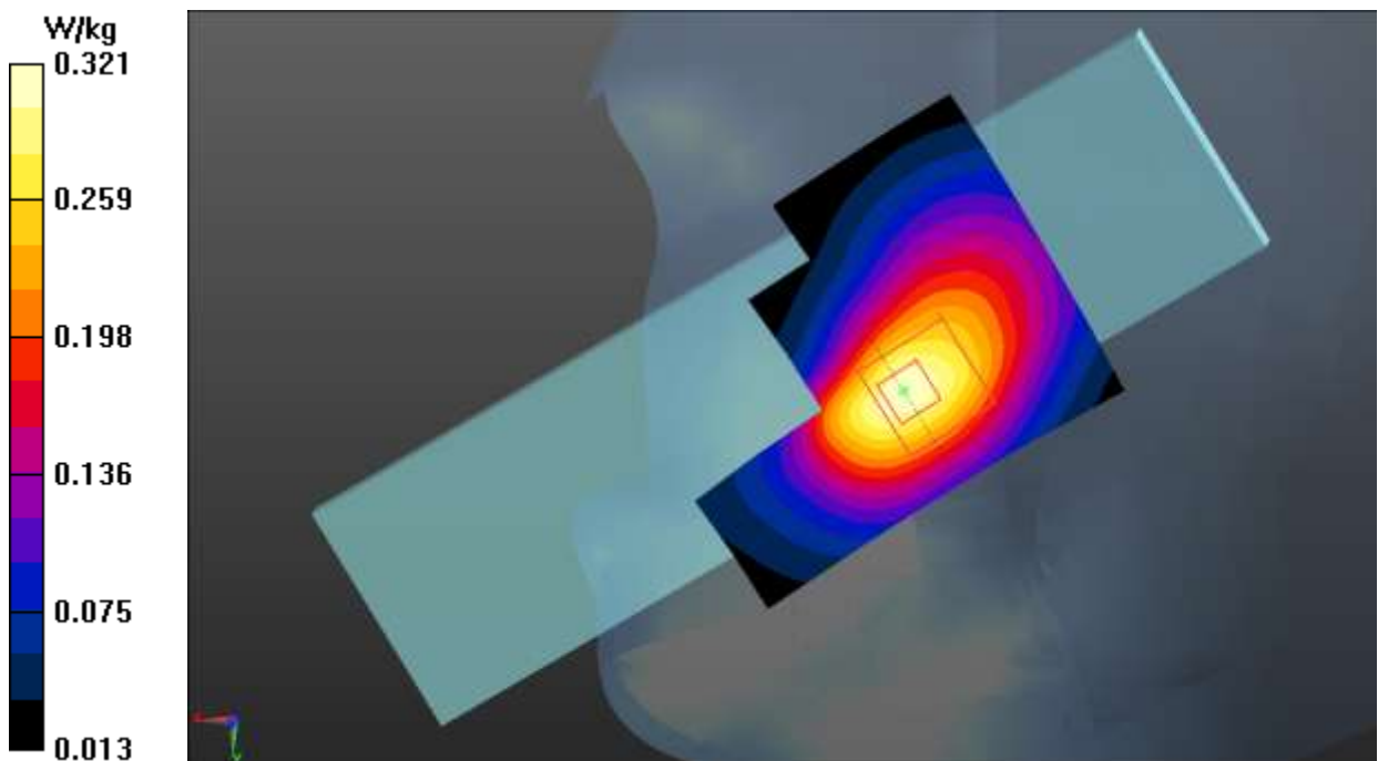
Fig.25 LTE Band 26
