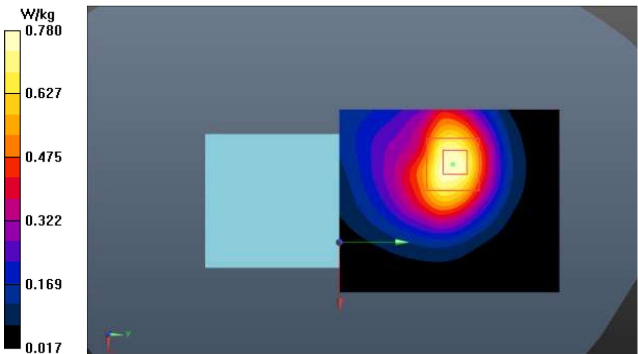
Fig.8 CDMA BC1
