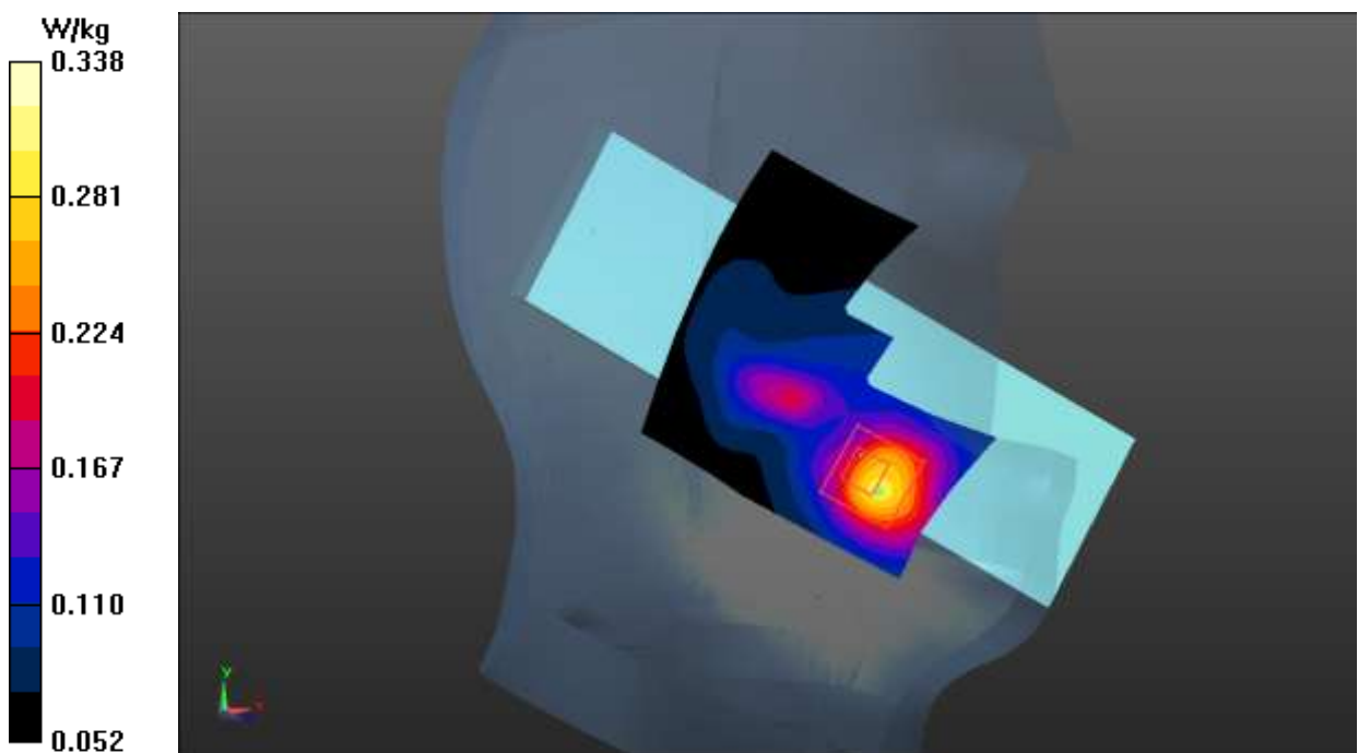
Fig.27 LTE Band 41
