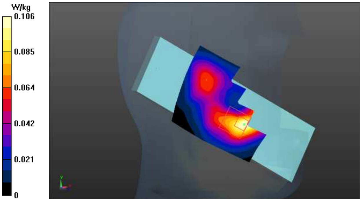
Fig.33 WLAN 2.4G
