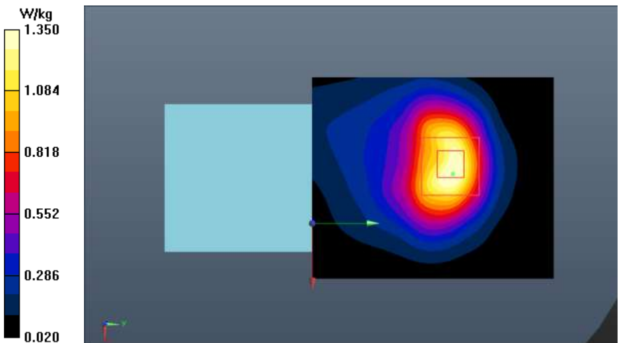
Fig.24 LTE Band 25
