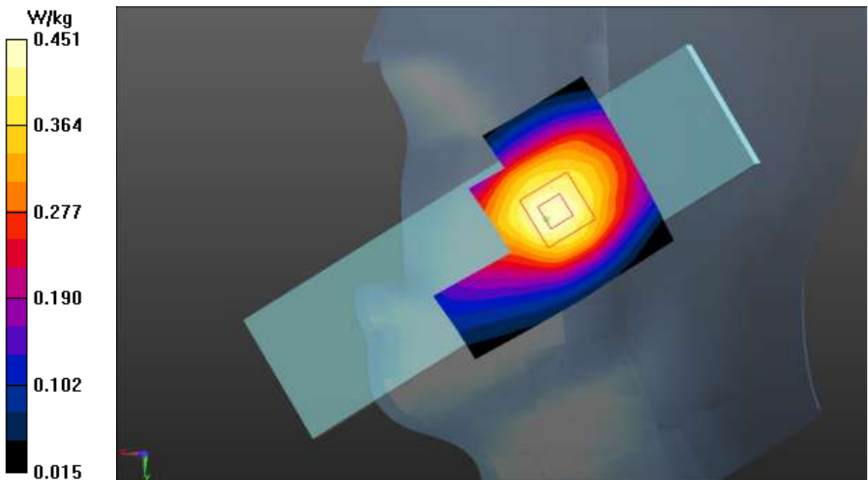
Fig.15 WCDMA Band 5
