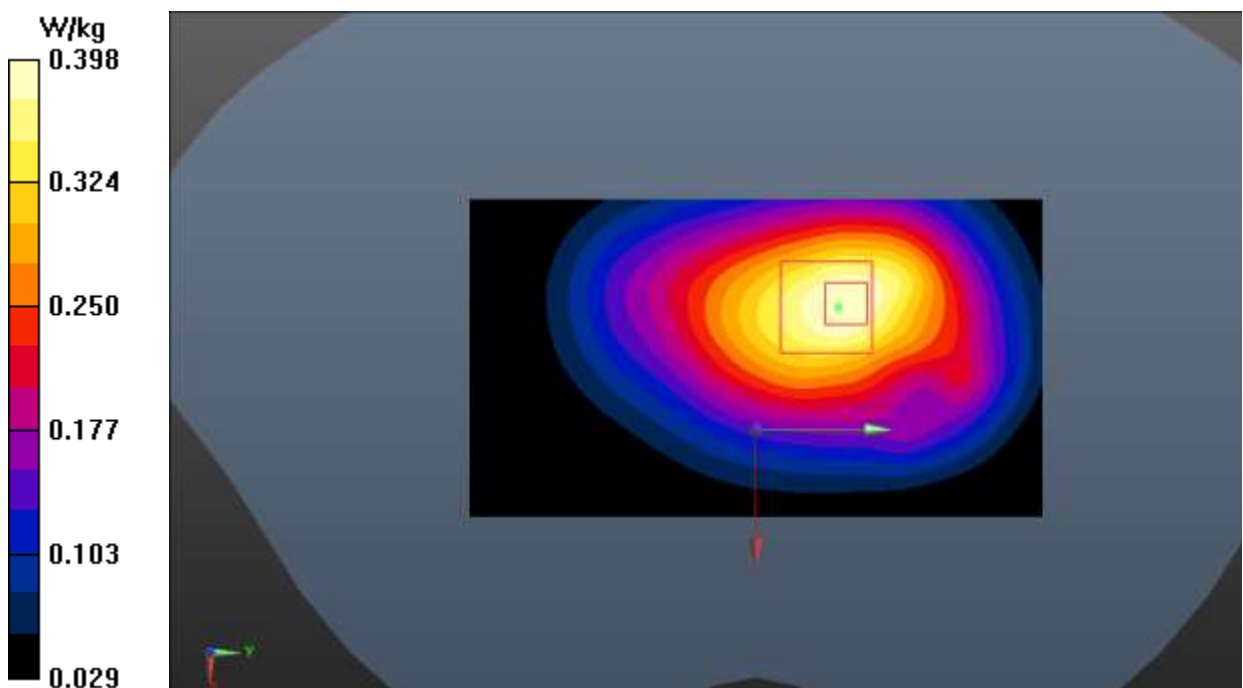
Fig.20 LTE Band 12
