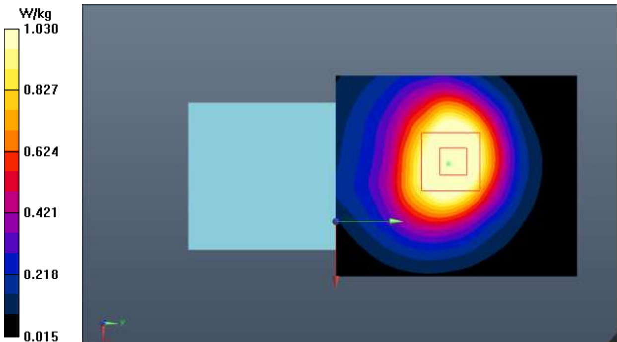
Fig.14 WCDMA Band 4
