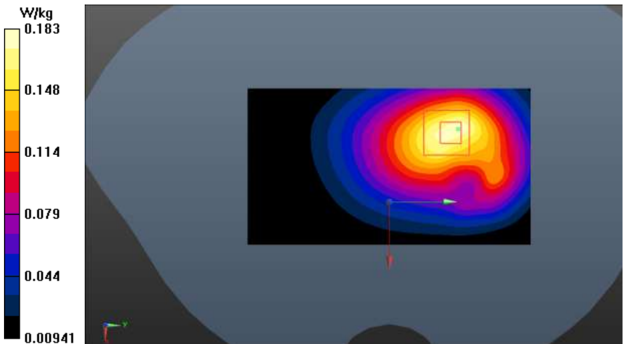
Fig.32 LTE Band 71
