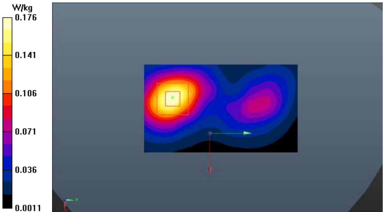
Fig.34 WLAN 2.4G
