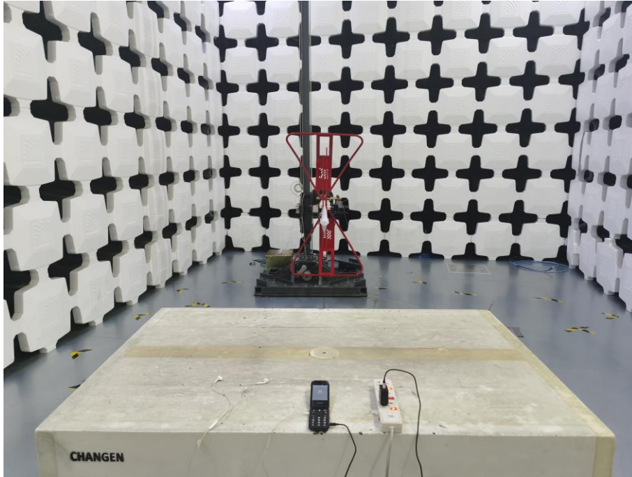
7. Radiated Emissions (Part 15B, FM receiver,30MHz-1GHz)
