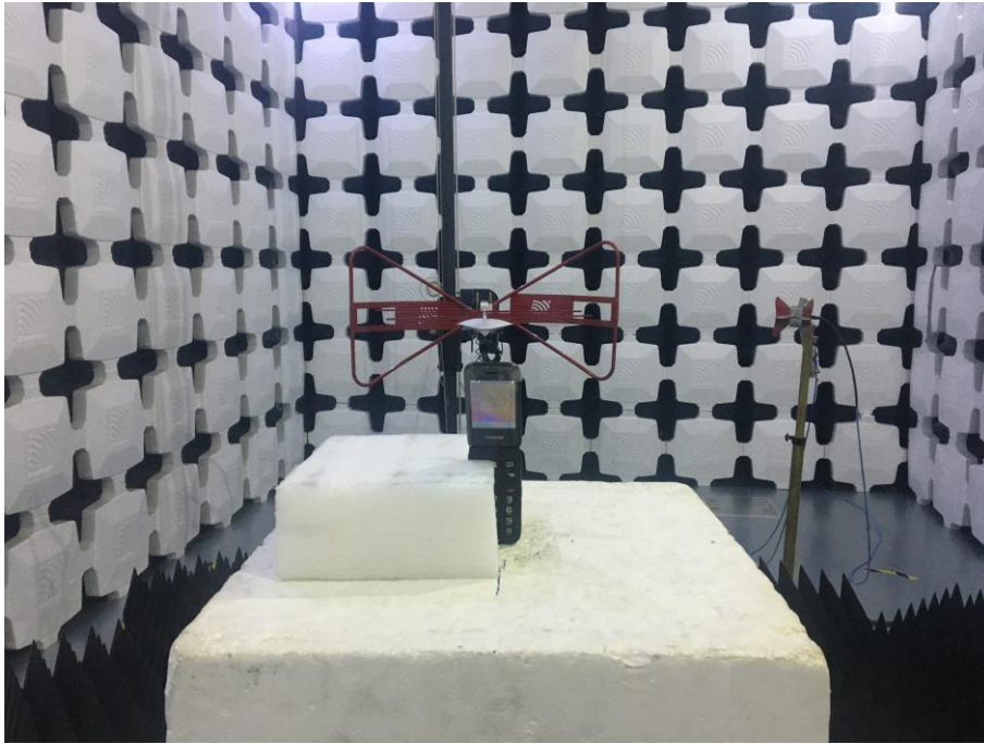
13. Radiated Emissions (Part 22/24/27/90,30MHz-18GHz)
