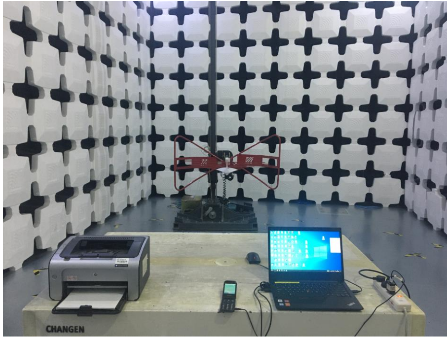
3. Radiated Emissions (Part 15B Bluetooth ,30MHz-1GHz)
