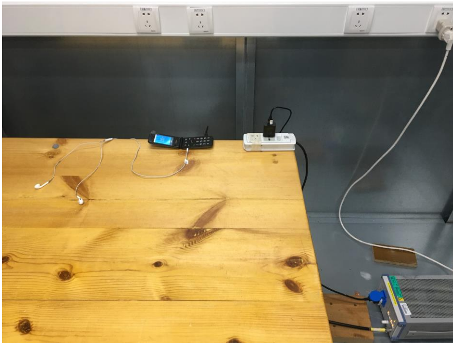
16. Conducted Emission (Part 15B, FM receiver)
