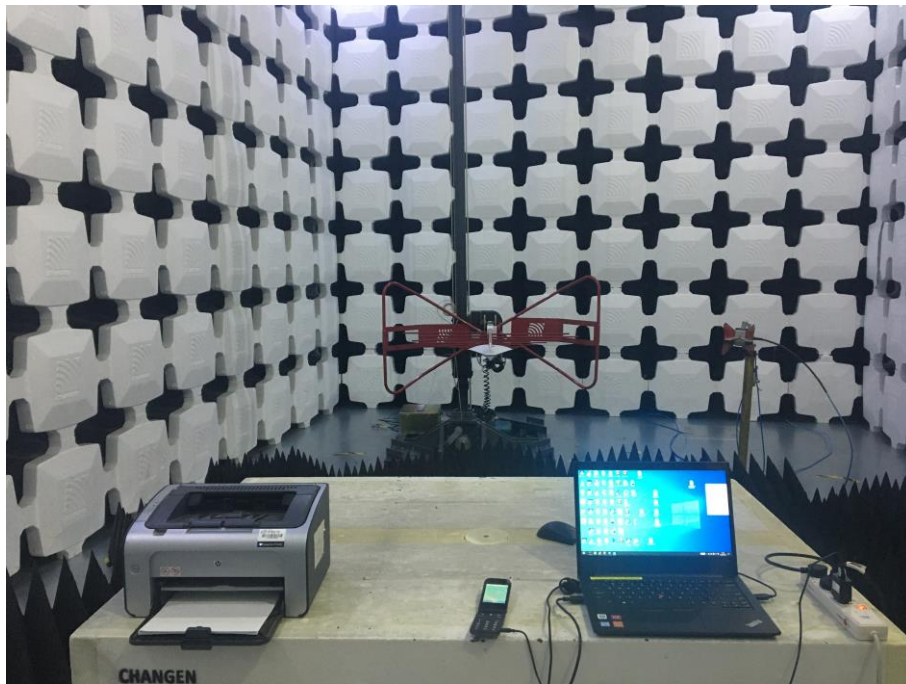
4. Radiated Emissions (Part 15B Bluetooth ,1GHz-18GHz)
