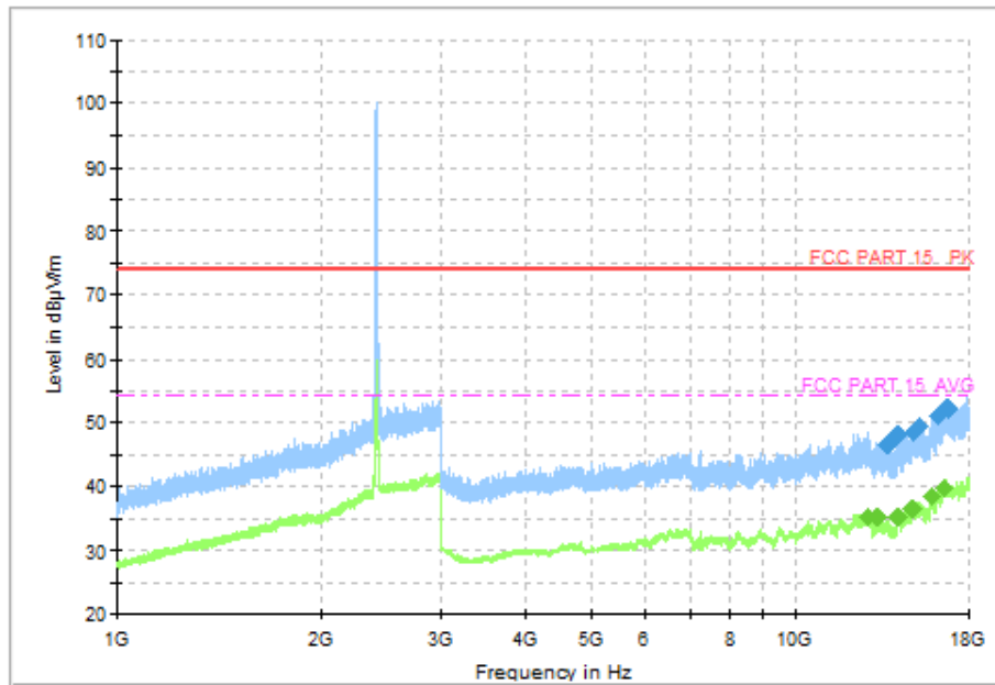
Fig.55 Radiated Spurious Emission (802.11n HT20, CH1, 1 GHz-18 GHz)
