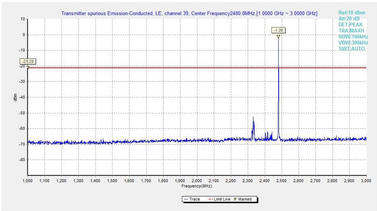
Fig.19 Conducted Spurious Emission (Ch39, 1 GHz-3 GHz)
