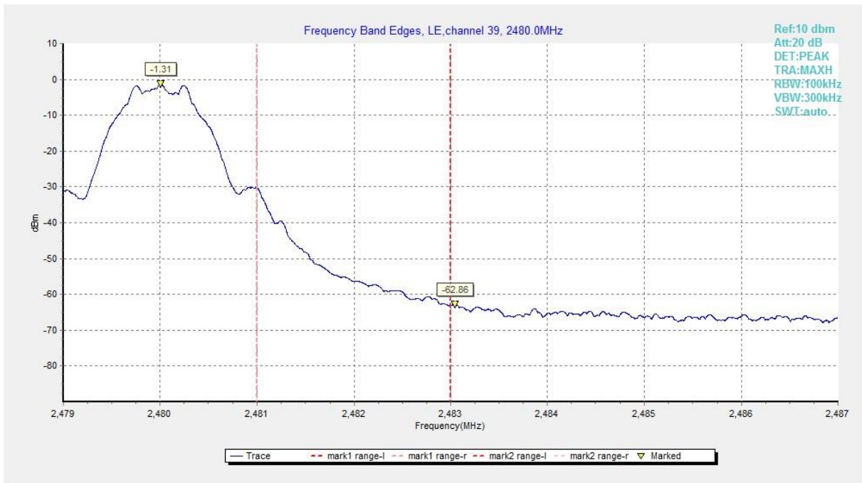
Fig.11 Band Edges (Ch 39)
