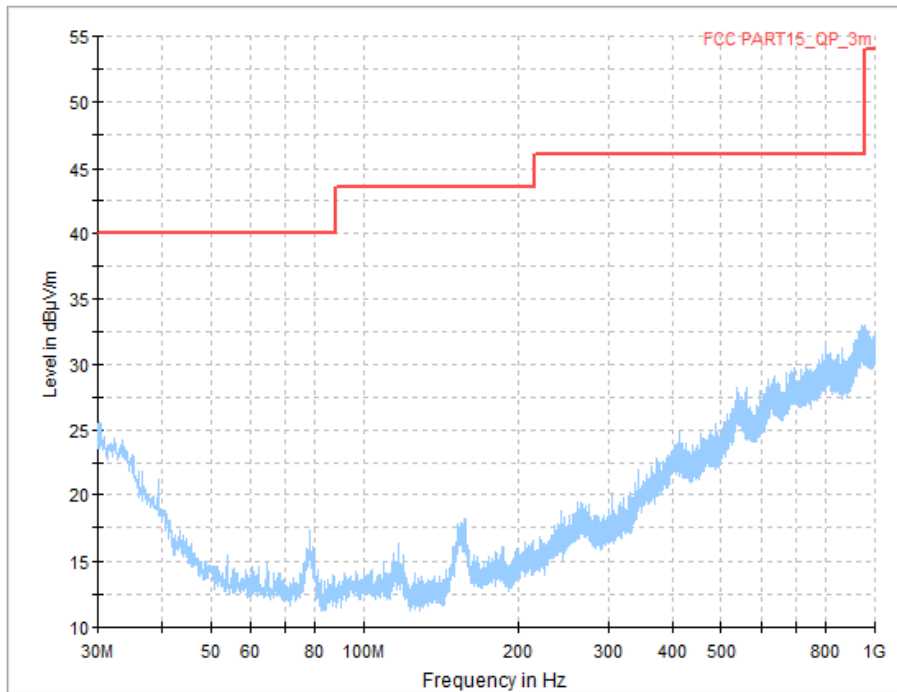
Fig.29 Radiated Spurious Emission (All Channels, 30 MHz-1 GHz)
