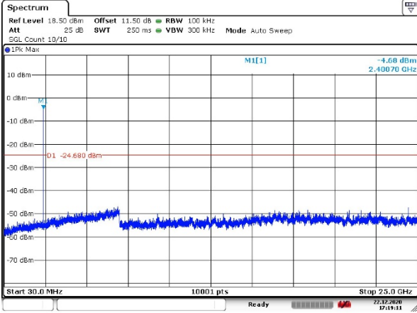
CH0 (Hopping off)
