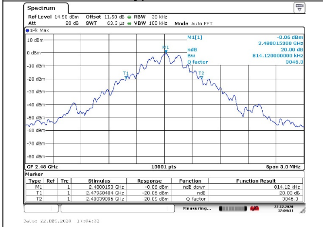
Modulation type: GFSK 2480MHz
