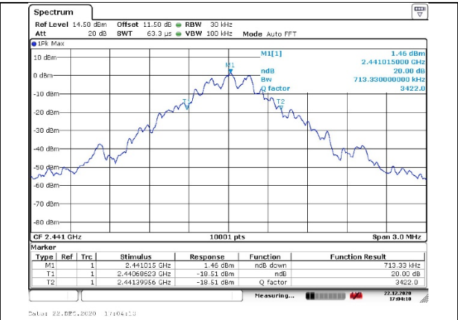
Modulation type: GFSK 2441MHz
