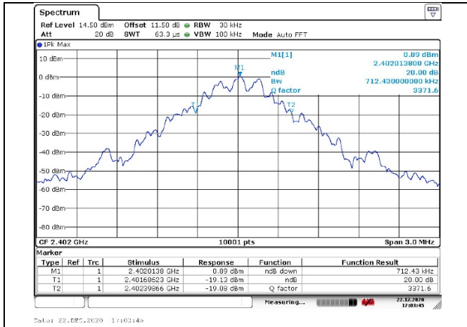
Modulation type: GFSK 2402MHz
