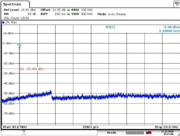
CH78 (Hopping off)
