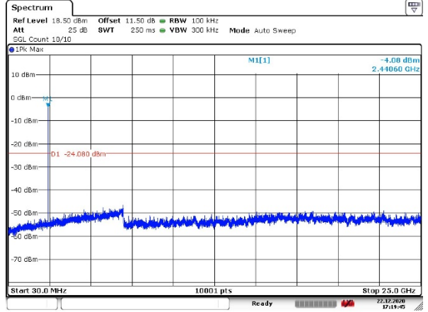
CH39 (Hopping off)
