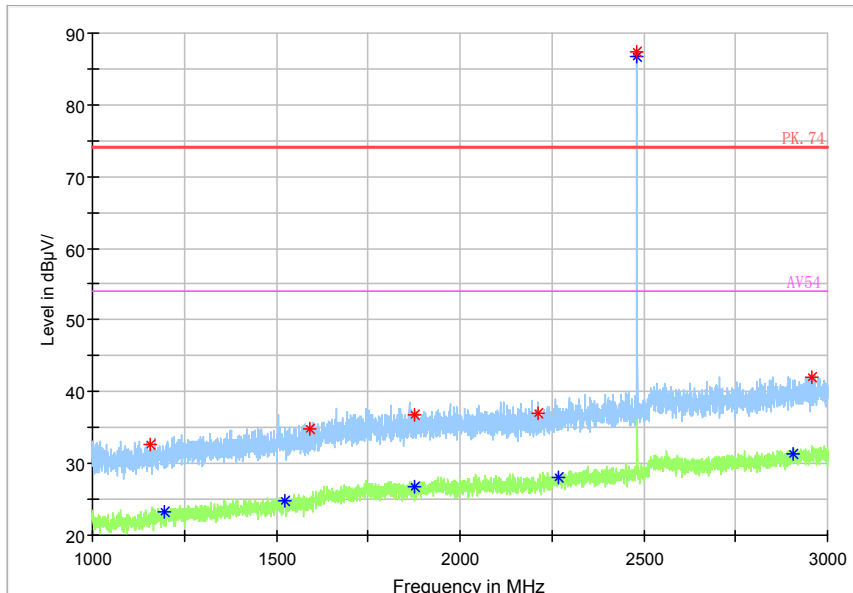
Frequency Range: 1GHz-3GHz Detector: Av mode and PK mode Modulation type: GFSK (LE)
