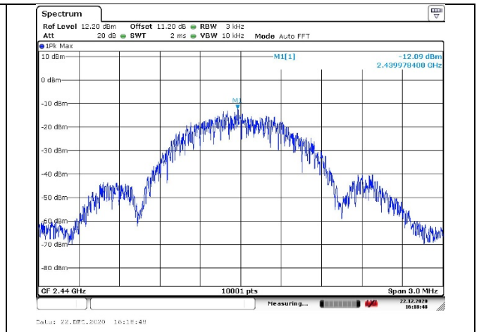
Modulation type: GFSK 2440MHz
