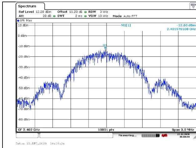
Modulation type: GFSK 2402MHz
