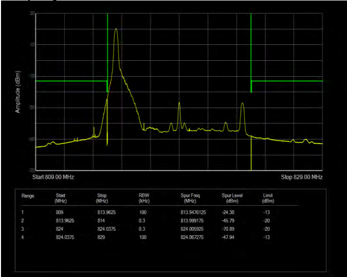
Band26(814-824) 16QAM BW=10MHz Channel=26740 RB Size=1 Position=#Max Extended
