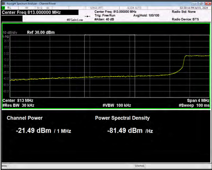
Band26(814-824) 16QAM BW=10MHz Channel=26740 RB Size=50 Position=#0 Normal
