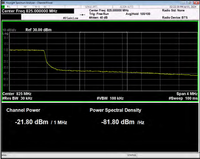
Band26(814-824) 16QAM BW=5MHz Channel=26765 RB Size=25 Position=#0 Normal
