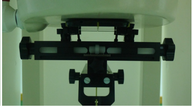
Back of the DUT with Phantom 0 cm Gap
