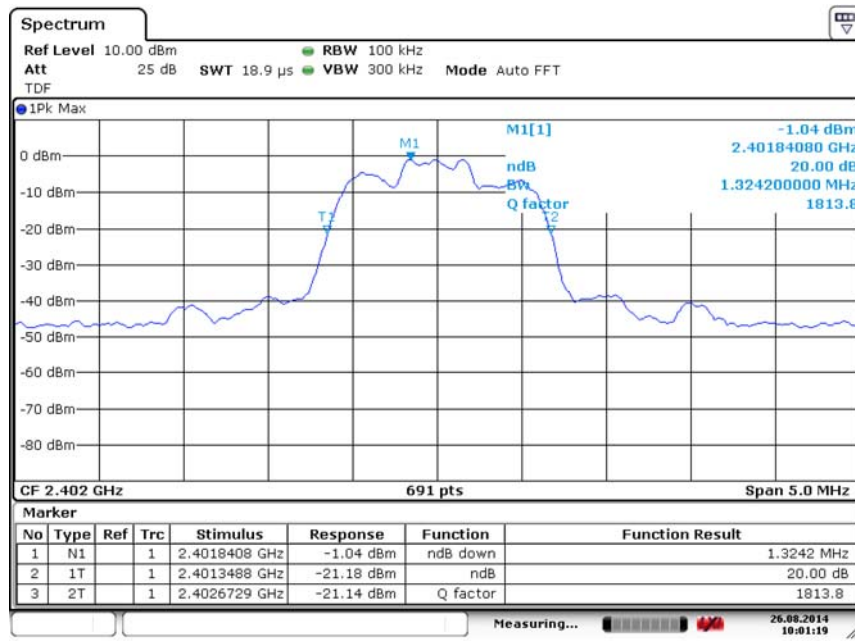
Fig. 81 Occupied 20dB Bandwidth (8DPSK, Ch 0)
