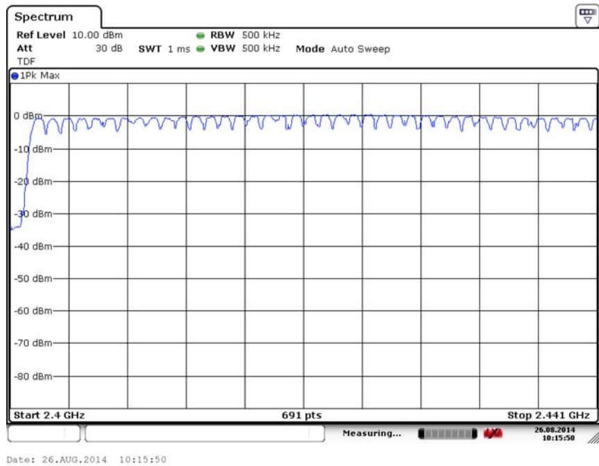
Fig. 92 Hopping channel ch0~39 ( \pi/4 DQPSK, Ch39)
