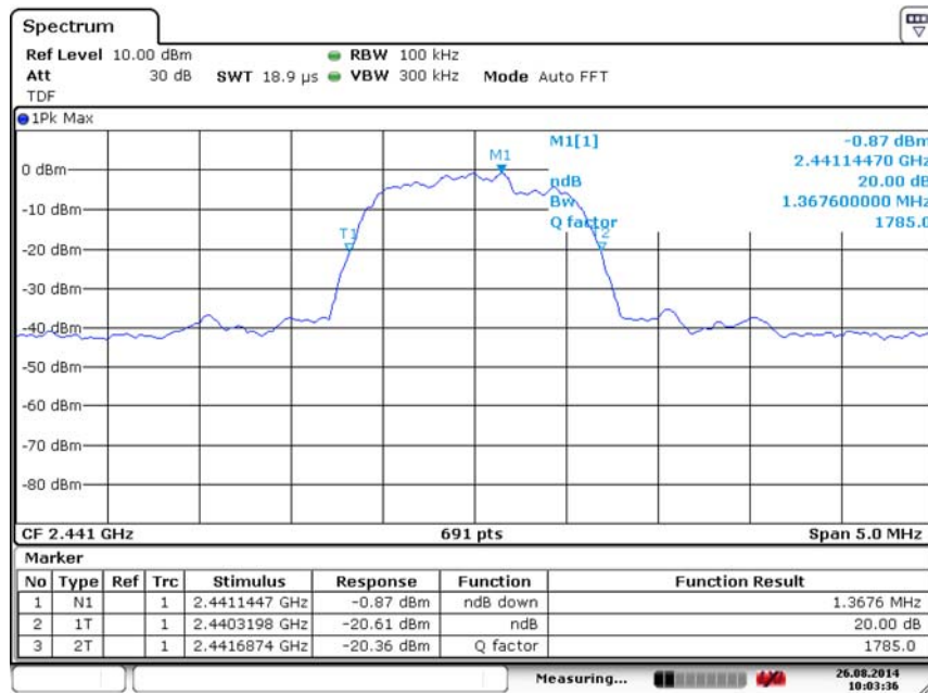
Fig. 82 Occupied 20dB Bandwidth (8DPSK, Ch 39)
