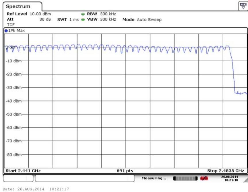
Fig. 91 Hopping channel ch39~78 (GFSK, Ch39)
