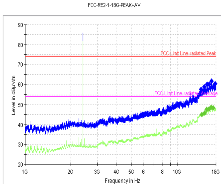
Fig. 67 Radiated Spurious Emission (8DPSK, Ch0, 1 GHz ~18 GHz)
