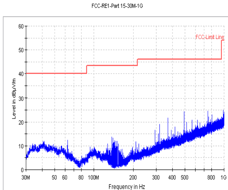
Fig. 70 Radiated Spurious Emission (8DPSK, Ch78, 30 MHz ~1 GHz)
