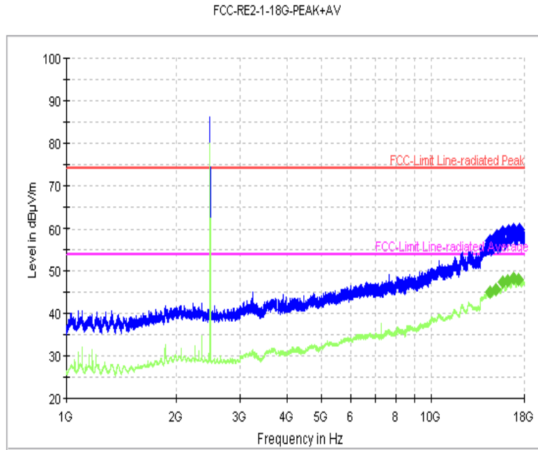
Fig. 27 Radiated Spurious Emission (Ch39, 1 GHz-18 GHz)
