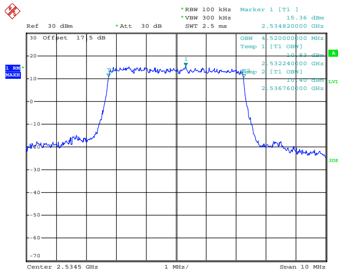
99% Occupied Bandwidth Plot on Channel 21095 for RB Size 25, RB Offset 0
