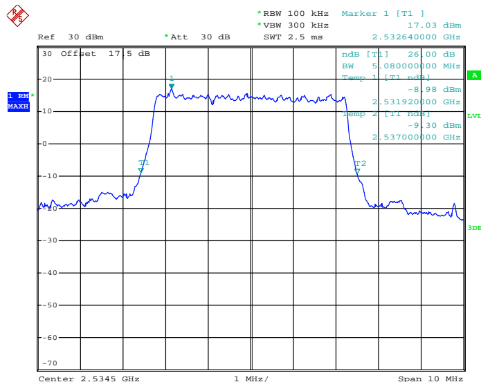
26dB Bandwidth Plot on Channel 21095 for RB Size 25, RB Offset 0
