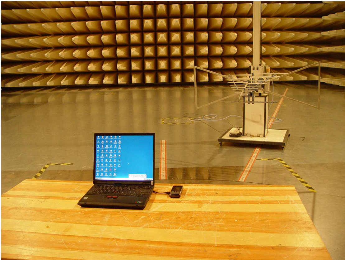
Pic 1 Radiated Emissions Test Setup
