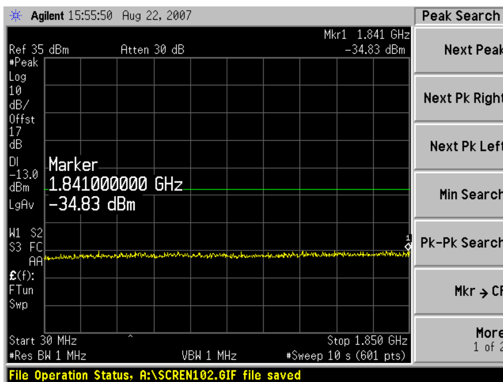
Channel 661, 30MHz~1850MHz
