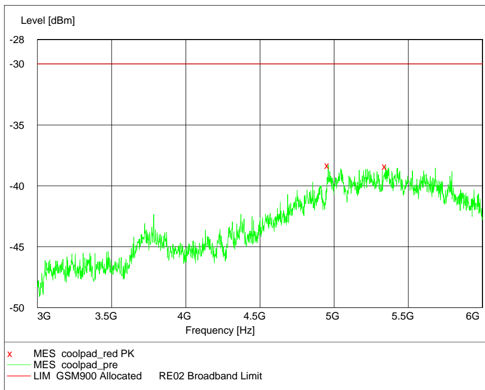
Channel 661, 3GHz~6GHz(Idle Mode)
