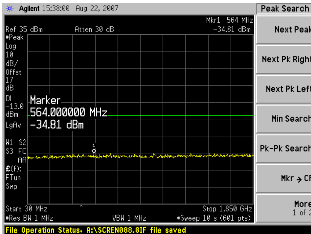
Channel 661, 30MHz~1850MHz
