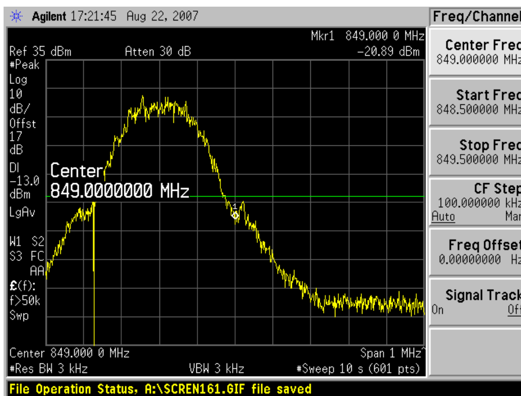
Channel 251
