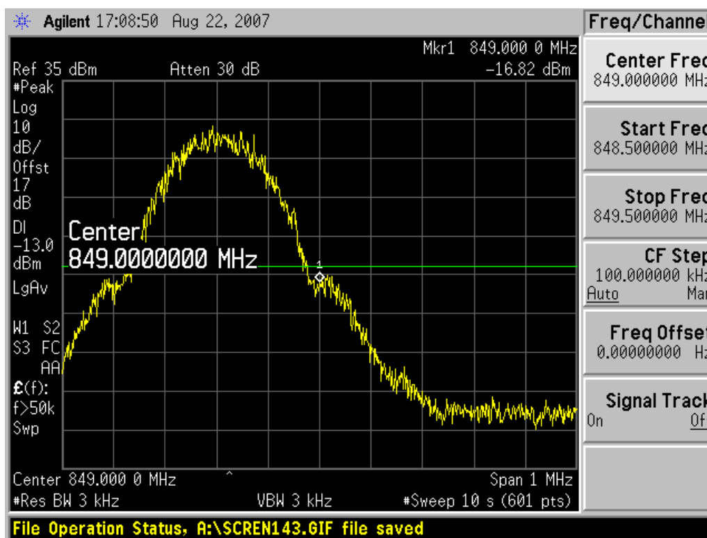
Channel 251
