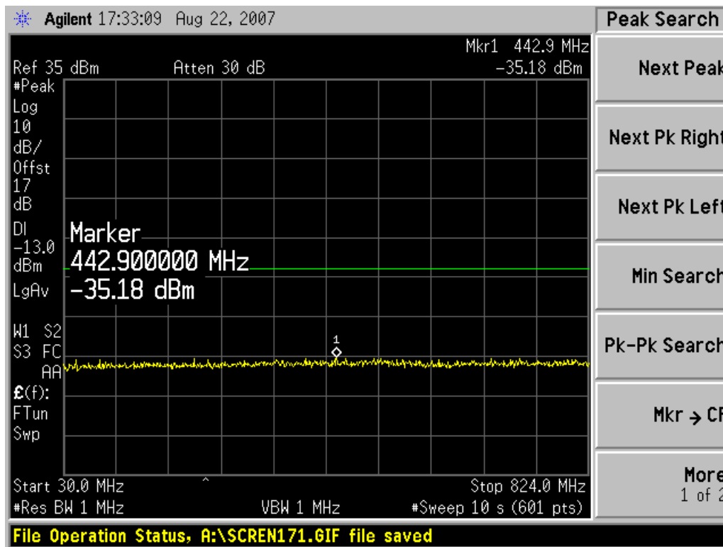
Channel 189, 30MHz~824MHz
