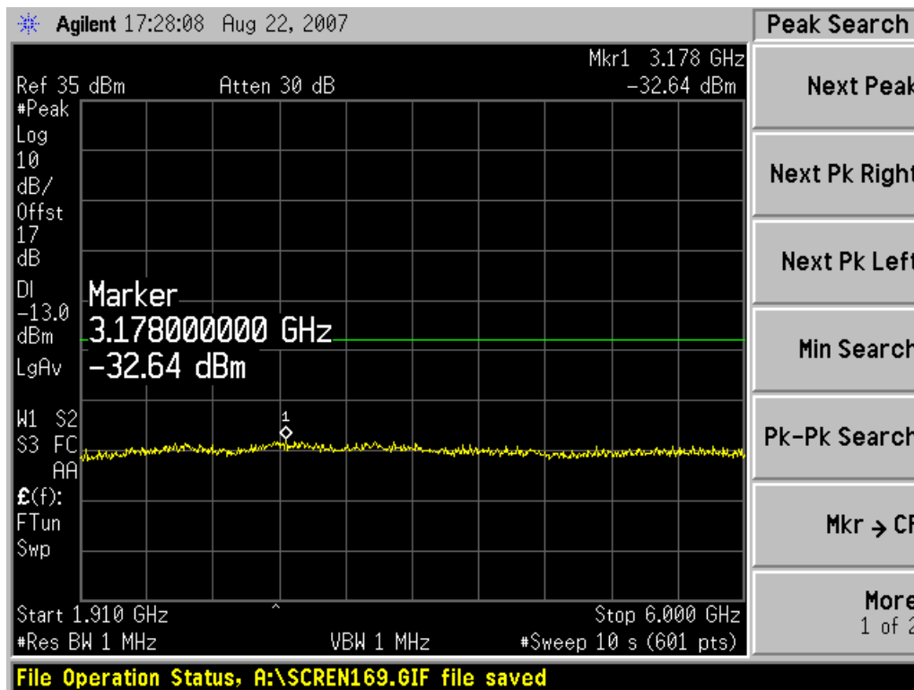
Channel 661, 1910MHz~6GHz
