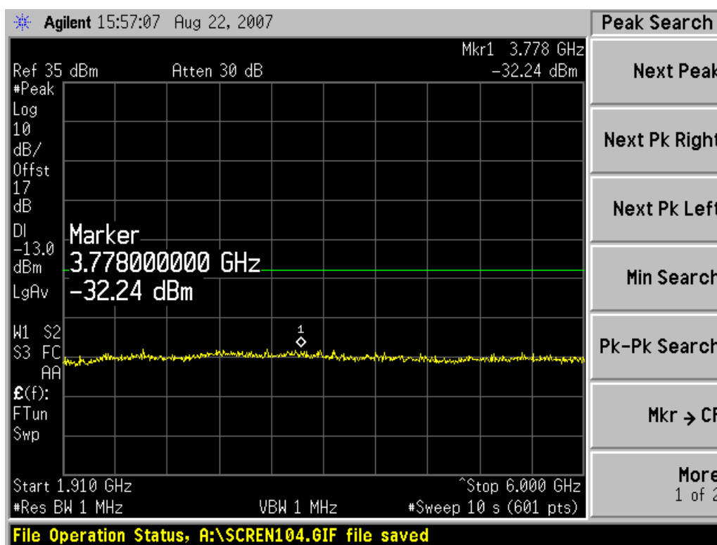
Channel 661, 1910MHz~6GHz
