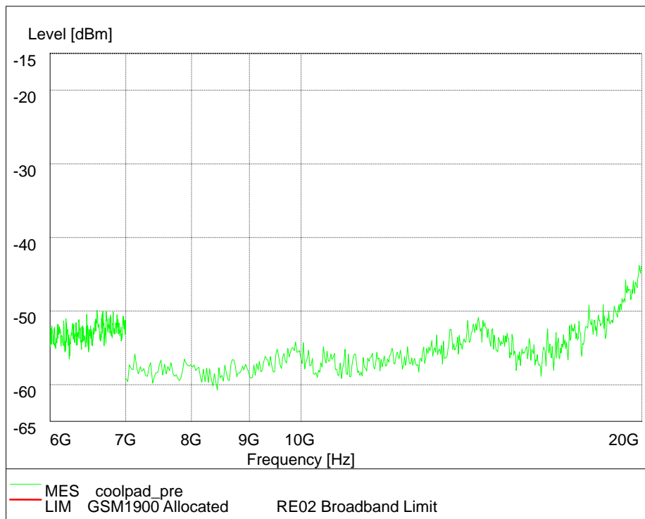
Channel 661, 6GHz~20GHz(Traffic Mode)
