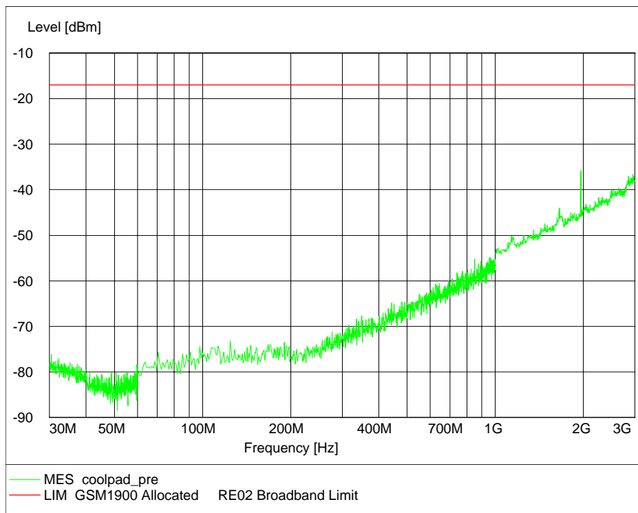
Channel 661, 30MHz~3GHz (Idle Mode)
