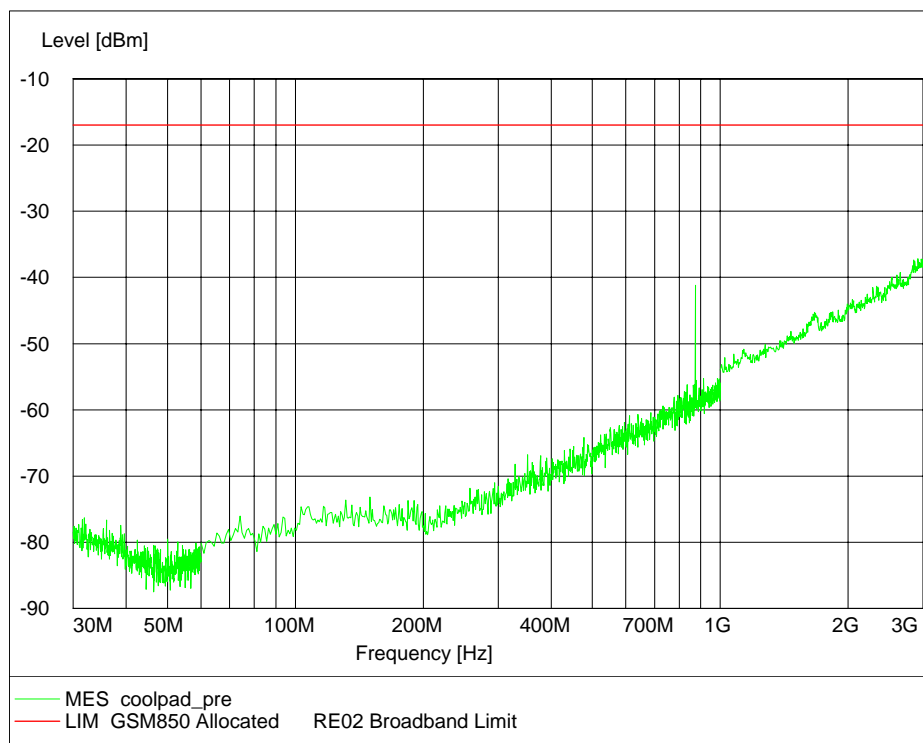
Channel 189, 30MHz~3GHz (Idle Mode)
