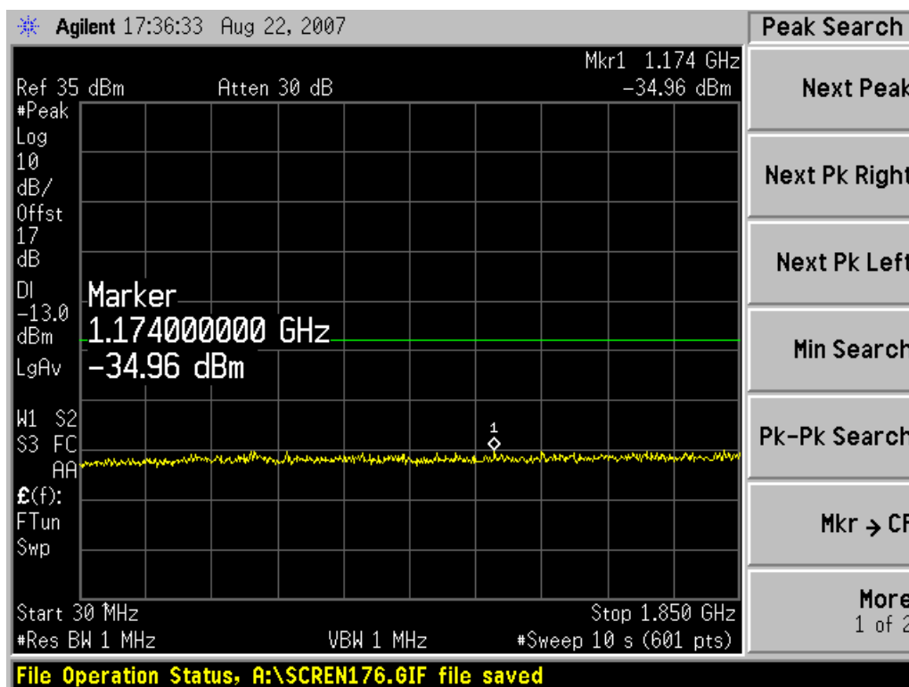
Channel 661, 30MHz~1850MHz
