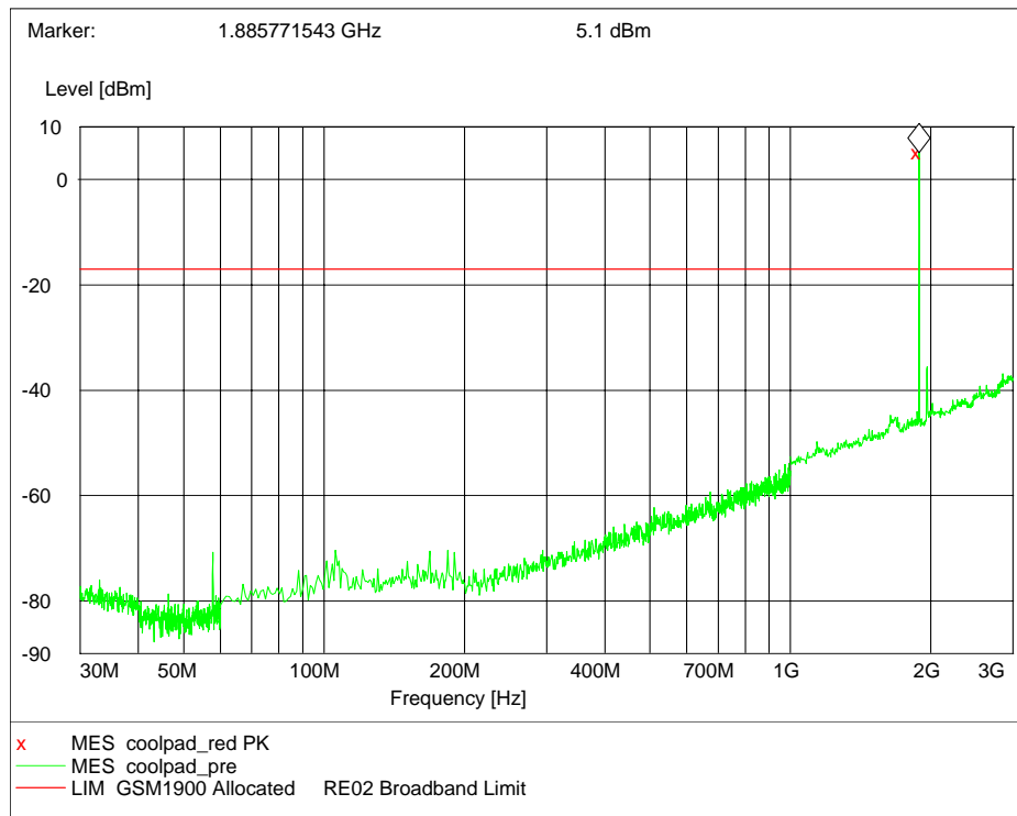
Channel 661, 30MHz~3GHz (Traffic Mode)
