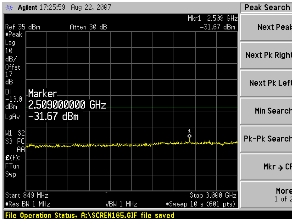
Channel 189, 849MHz~3GHz
