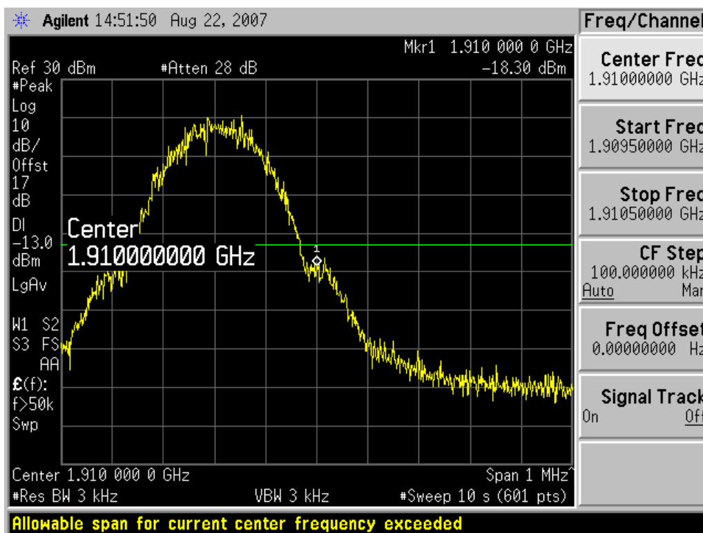
Channel 810
