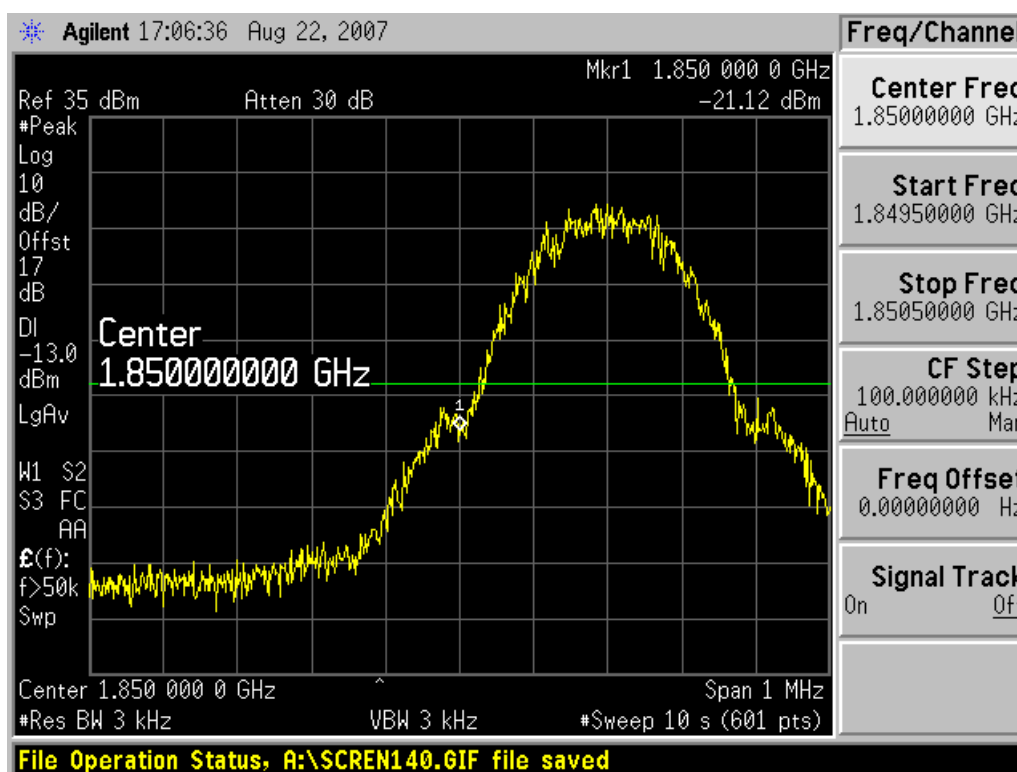
Channel 512
