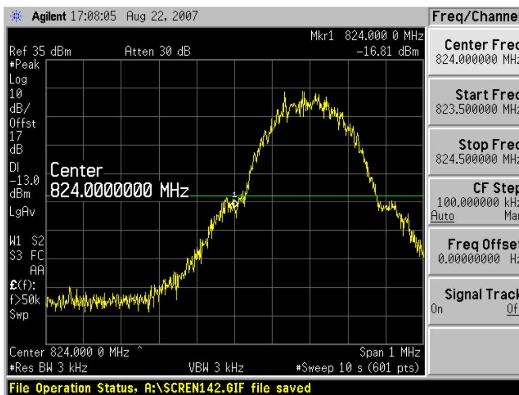
Channel 128
