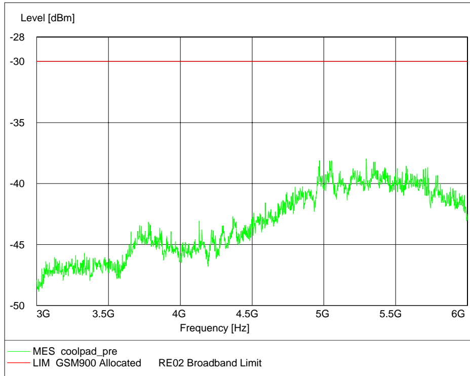
Channel 661, 3GHz~6GHz(Idle Mode)
