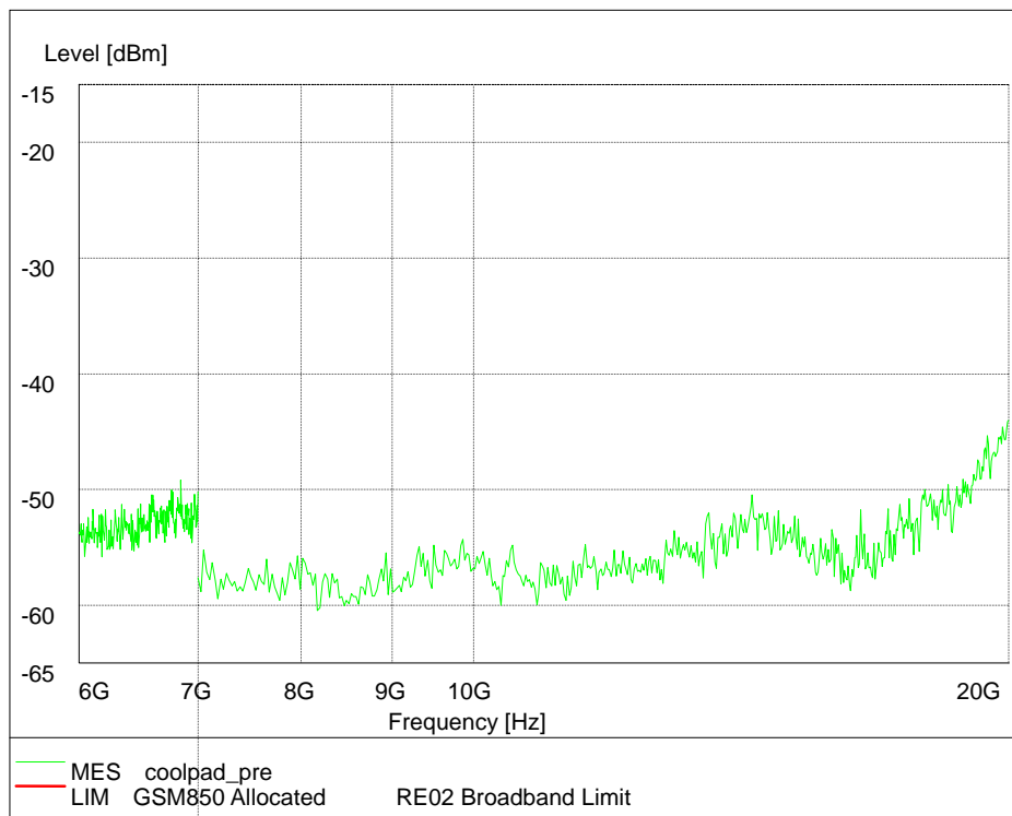
Channel 189, 6GHz~20GHz(Idle Mode)
