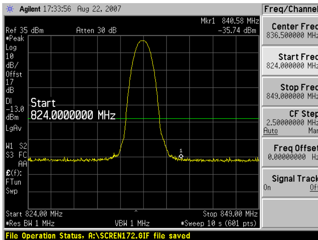
Channel 189, 824MHz~849MHz
