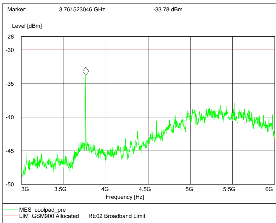
Channel 661, 3GHz~6GHz(Traffic Mode)
