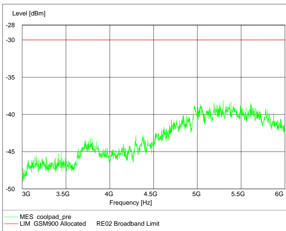
Channel 189, 3GHz~6GHz (Traffic Mode)
