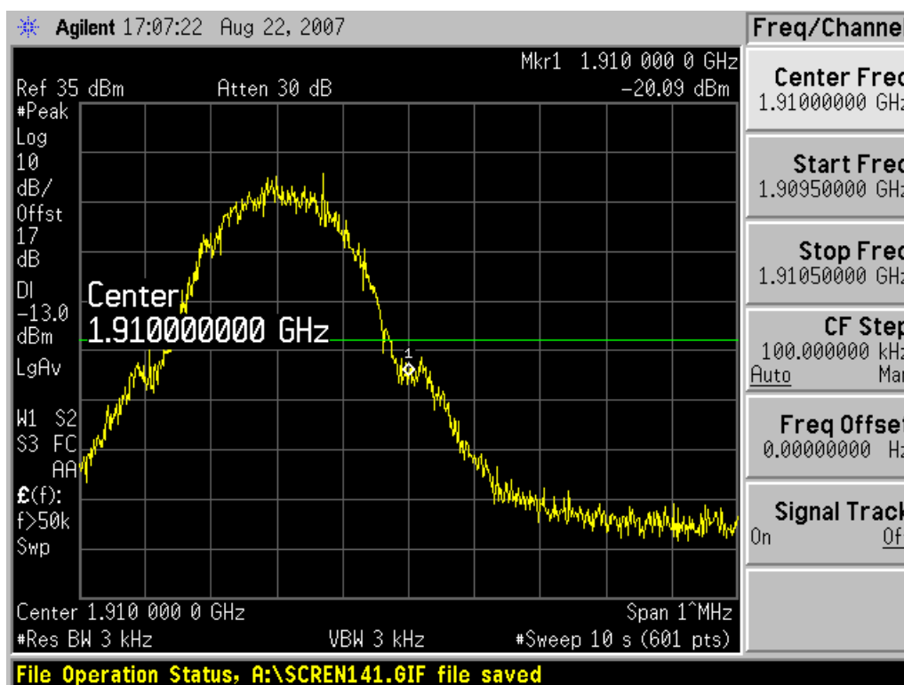
Channel 810
