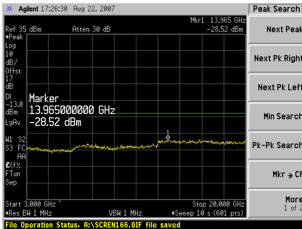
Channel 189, 3GHz~20GHz
