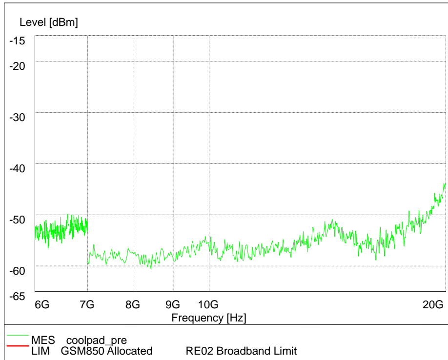
Channel 189, 6GHz~20GHz (Traffic Mode)
