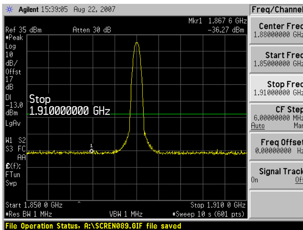
Channel 661, 1850MHz~1910MHz
