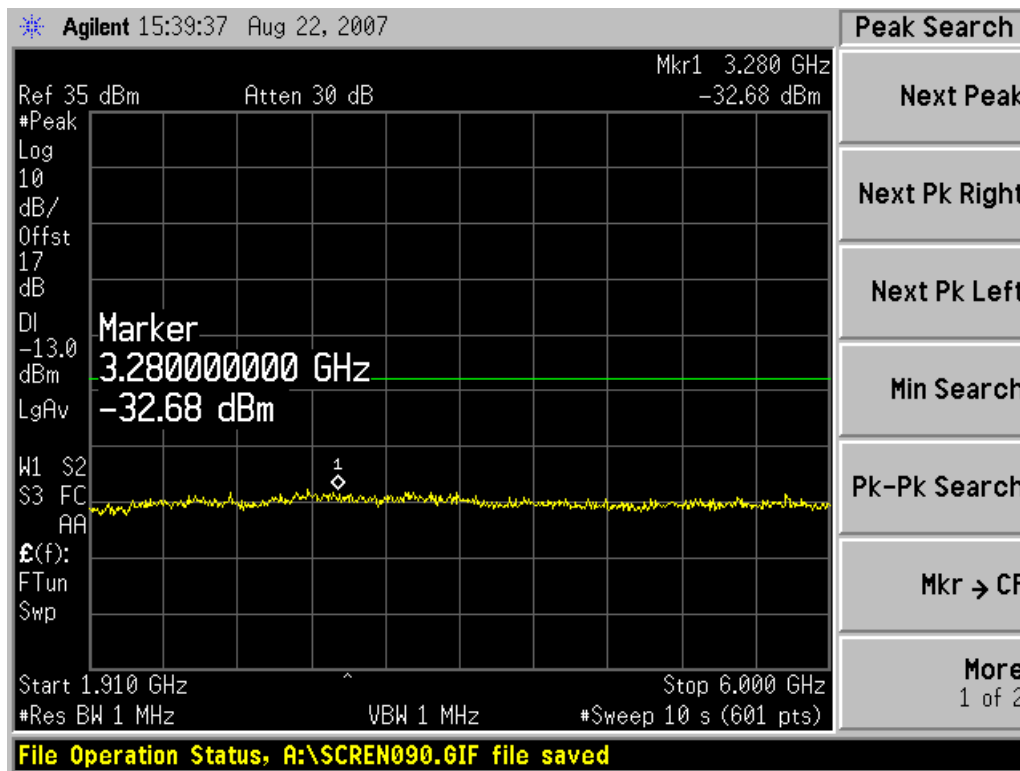
Channel 661, 1910MHz~6GHz
