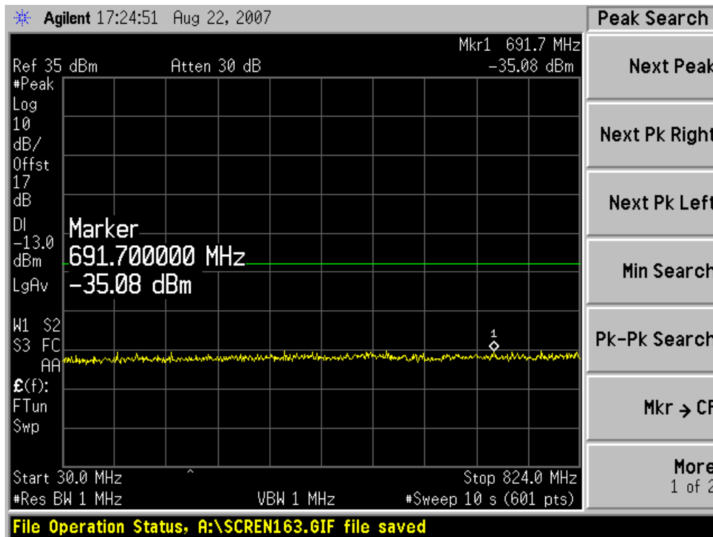
Channel 189, 30MHz~824MHz
