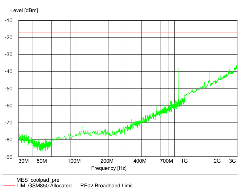
Channel 189, 30MHz~3GHz (Traffic Mode)
