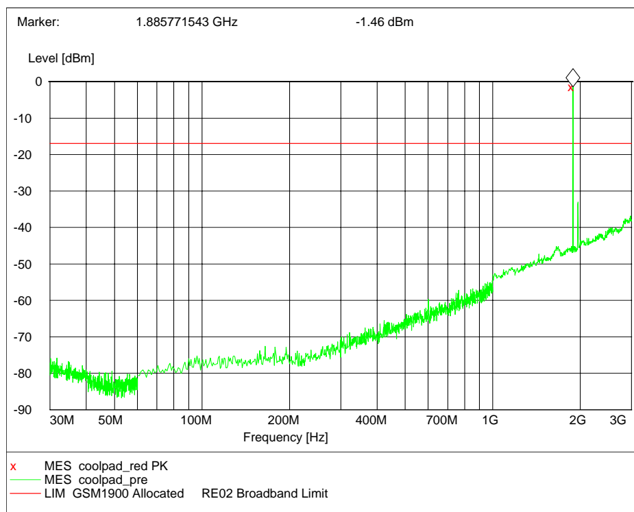
Channel 661, 30MHz~3GHz (Traffic Mode)
