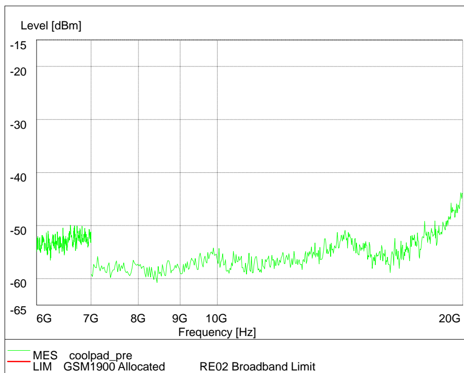
Channel 661, 6GHz~20GHz(Idle Mode)
