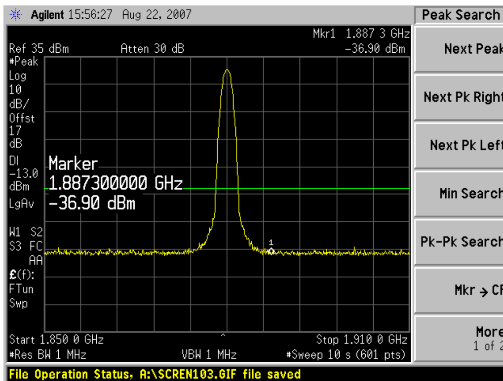
Channel 661, 1850MHz~1910MHz
