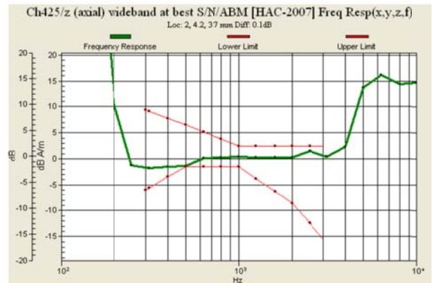
Fig. 9.2 CDMA2000 BC15 Ch425
