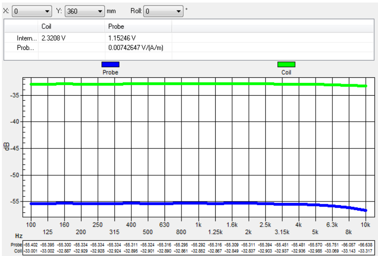
Fig. 5.2 The frequency response and sensitivity of AM1D probe
