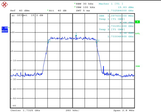
3RB Size, RB Offset 2, QPSK
