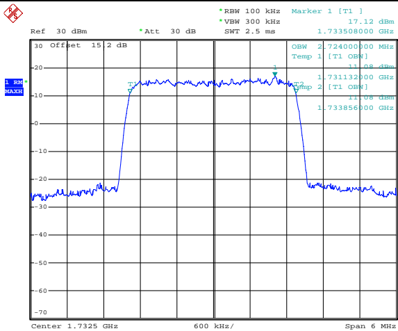
8RB Size, RB Offset 4, QPSK
