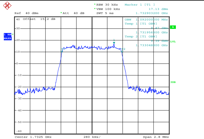
3RB Size, RB Offset 2, 16QAM
