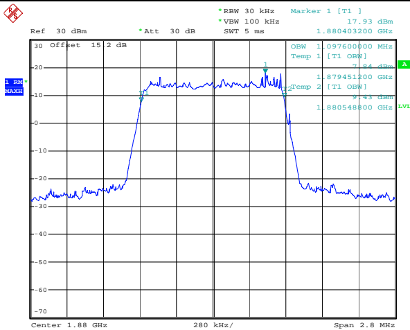
3RB Size, RB Offset 2, QPSK
