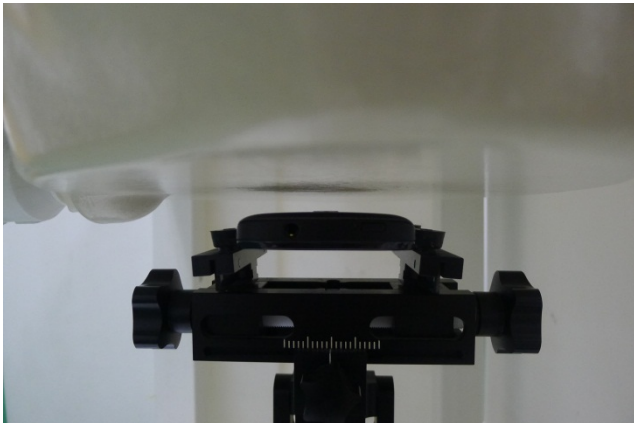
Back of the DUT with Phantom 1.0 cm Gap
