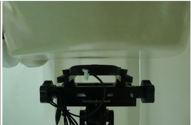
Back of the DUT with Phantom 1.0 cm Gap (With Earphone)
