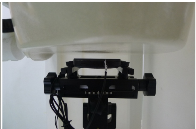
Front of the DUT with Phantom 1.0 cm Gap (With Earphone)
