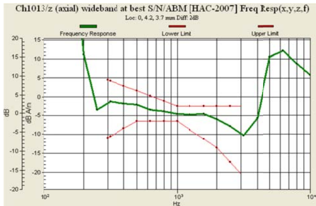
Fig. 9.1 CDMA2000 BC0 Ch1013
