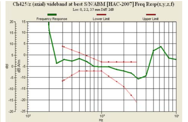
Fig. 9.8 CDMA2000 BC15 Ch425
