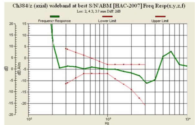
Fig. 9.2 CDMA2000 BC0 Ch384
