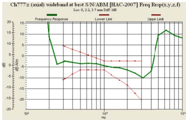
Fig. 9.3 CDMA2000 BC0 Ch777
