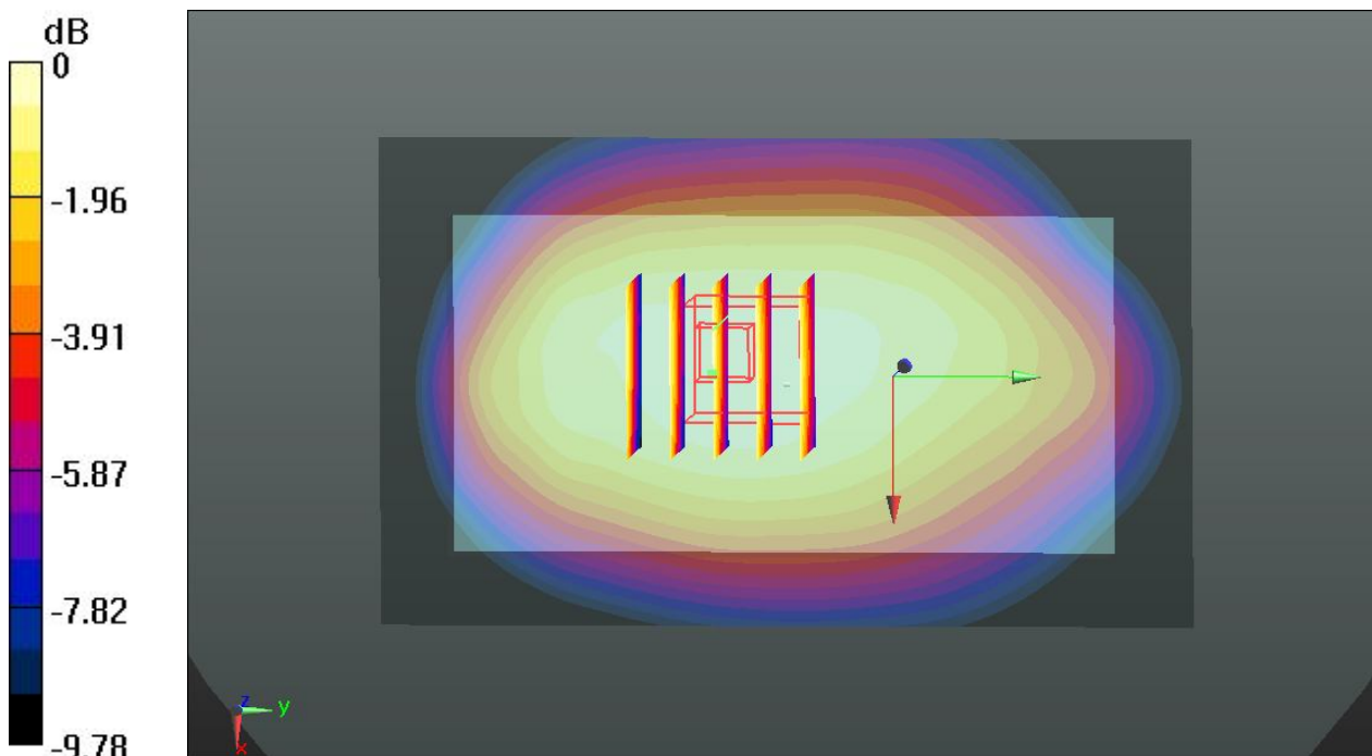
0 dB = 0.988 W/kg
