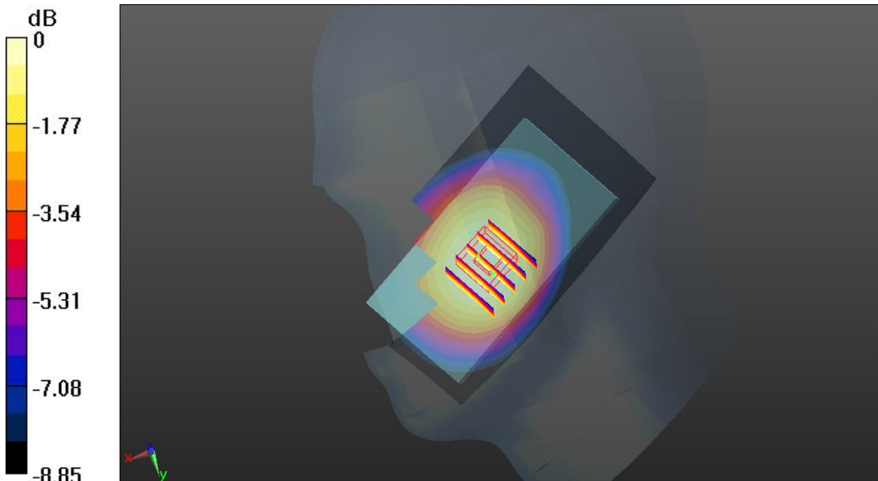
0 dB = 0.705 W/kg
