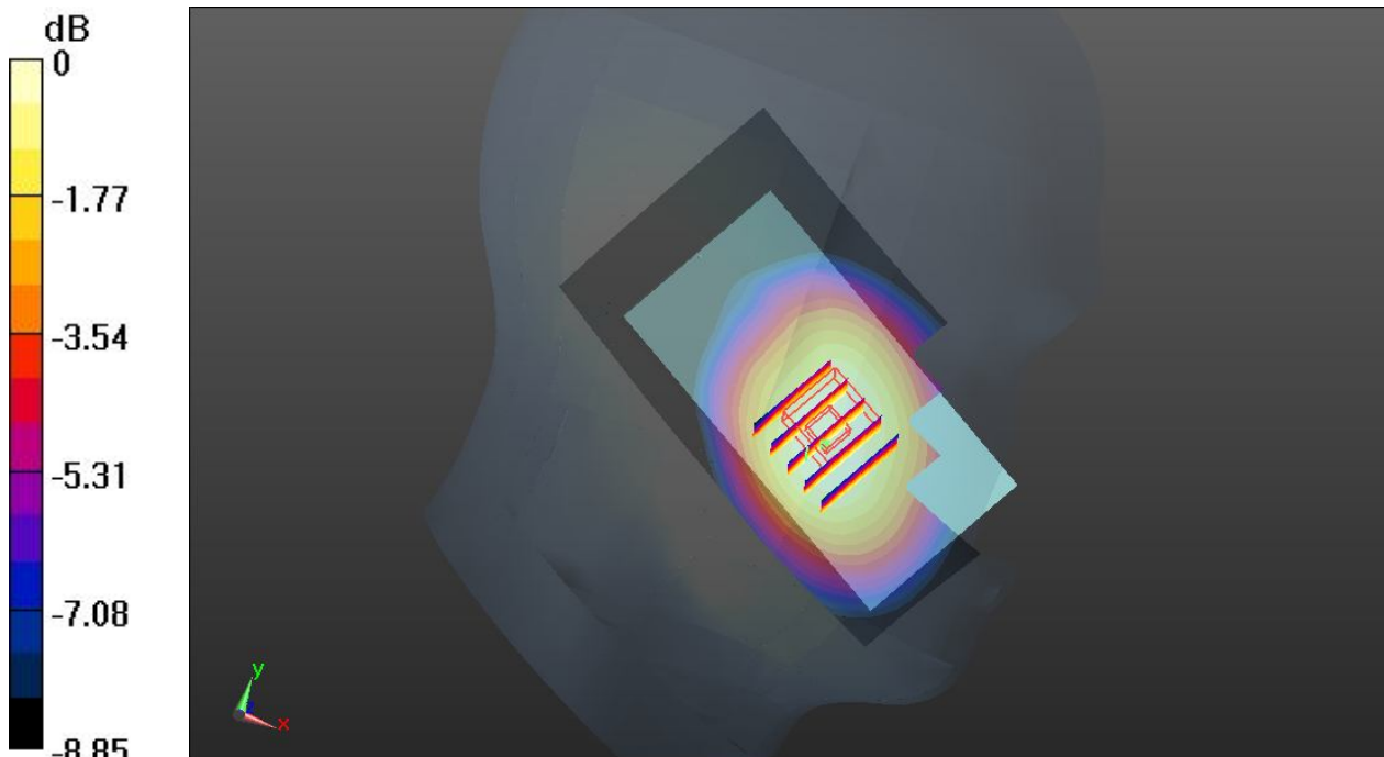
0 dB = 0.634 W/kg
