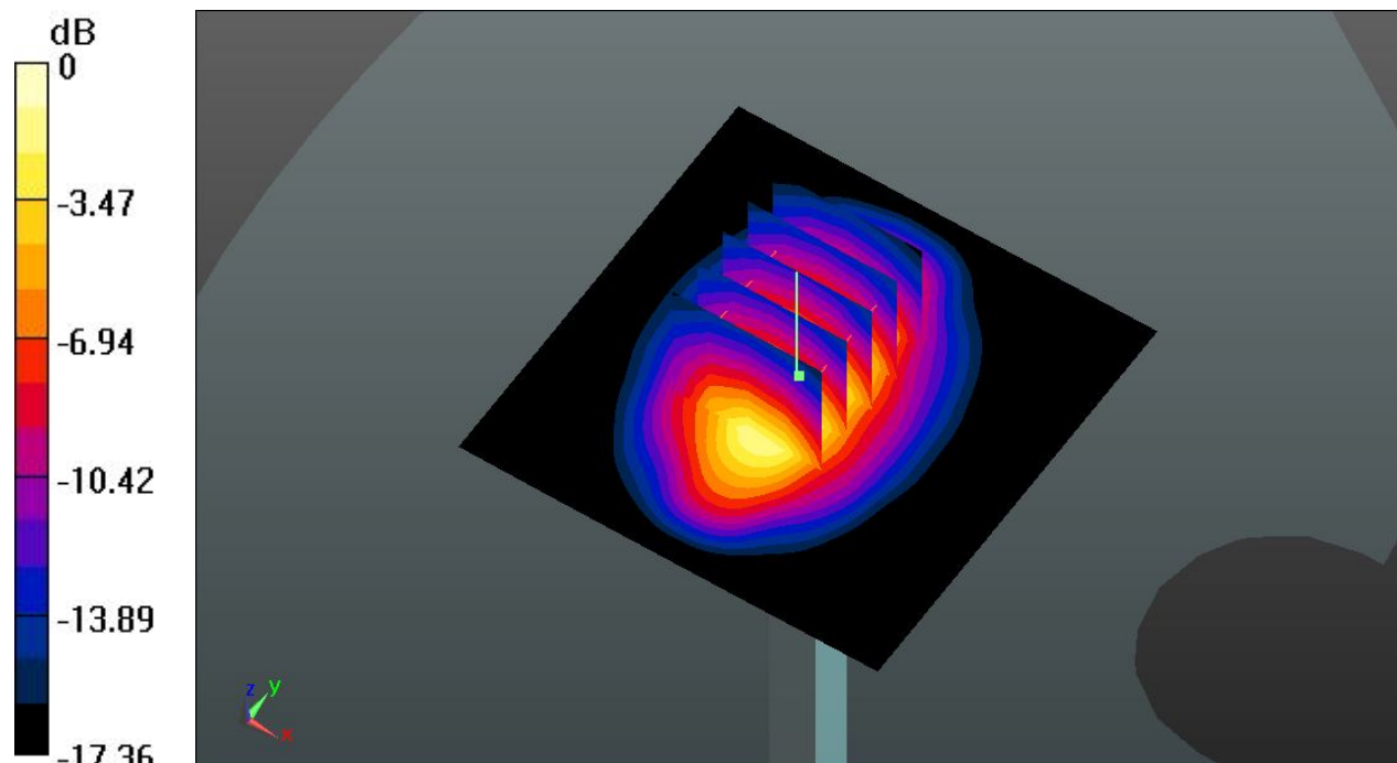
0 dB = 14.9 W/kg
