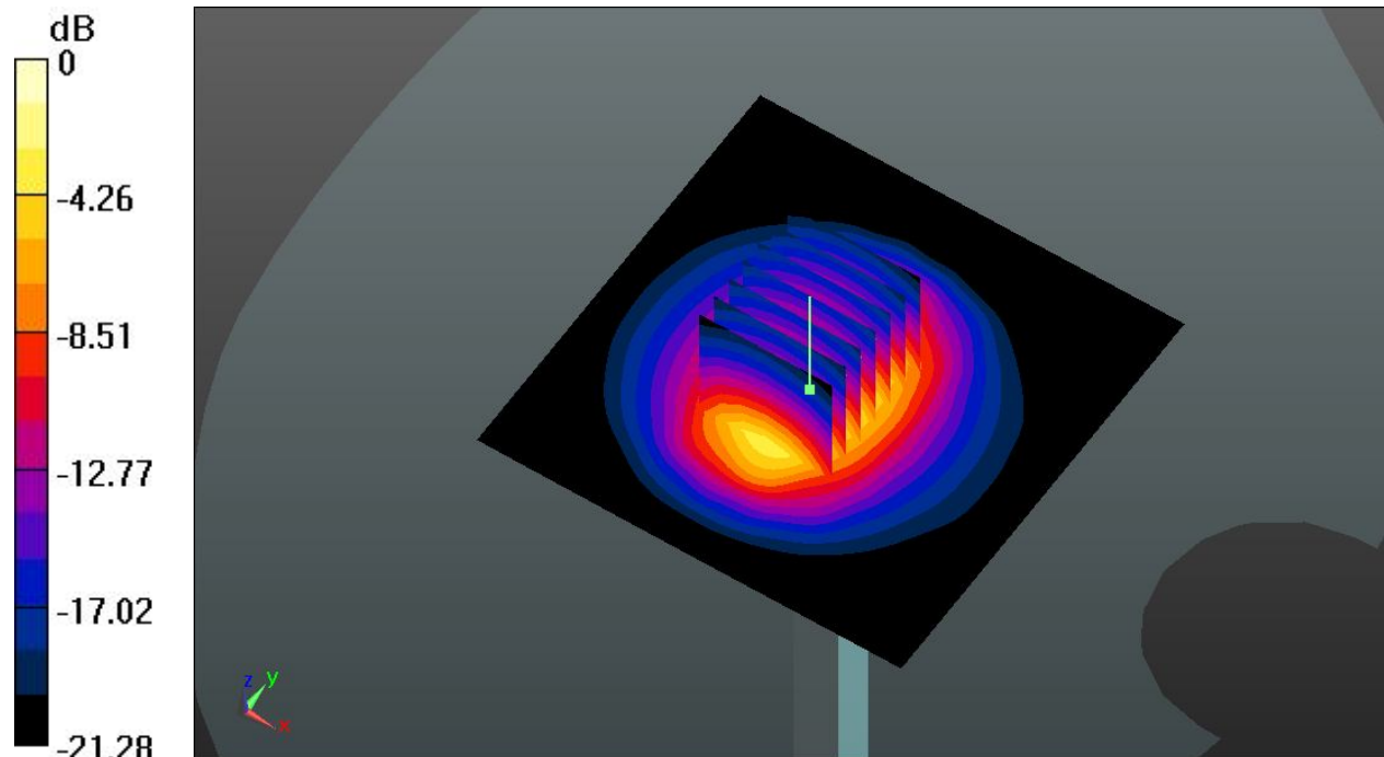
0 dB = 19.3 W/kg
