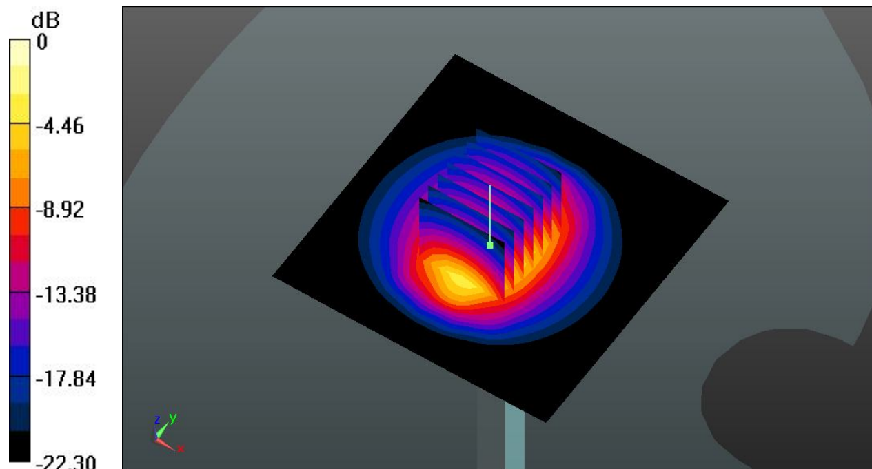
0 dB = 20.2 W/kg
