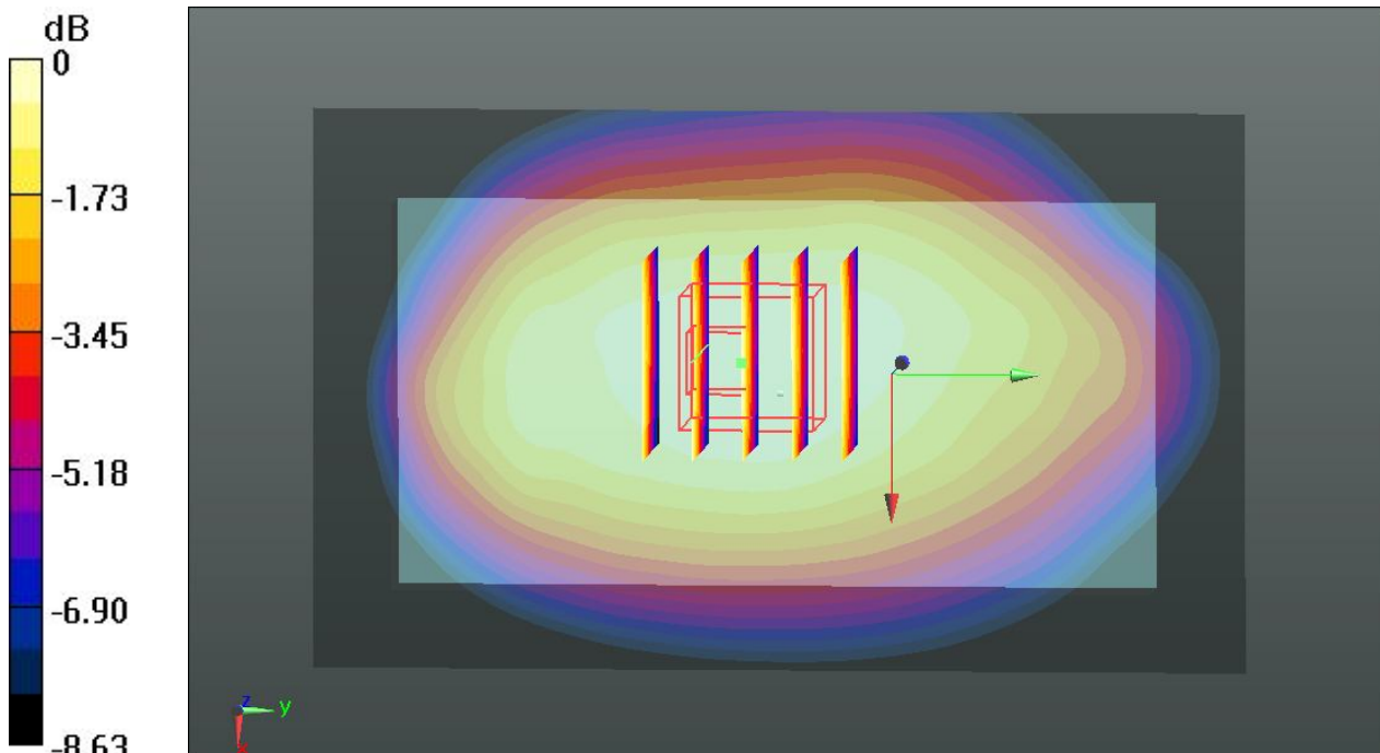
0 dB = 0.972 W/kg
