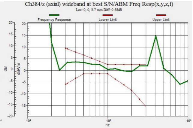
Fig 7.2 CDMA2000 BC0 Ch384
