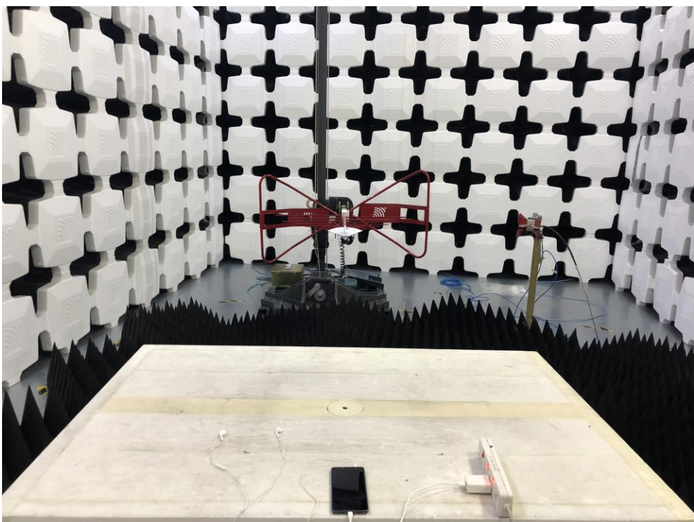
6. Radiated Emissions (Part 15B Charging mode-FM) (1-18GHz)
