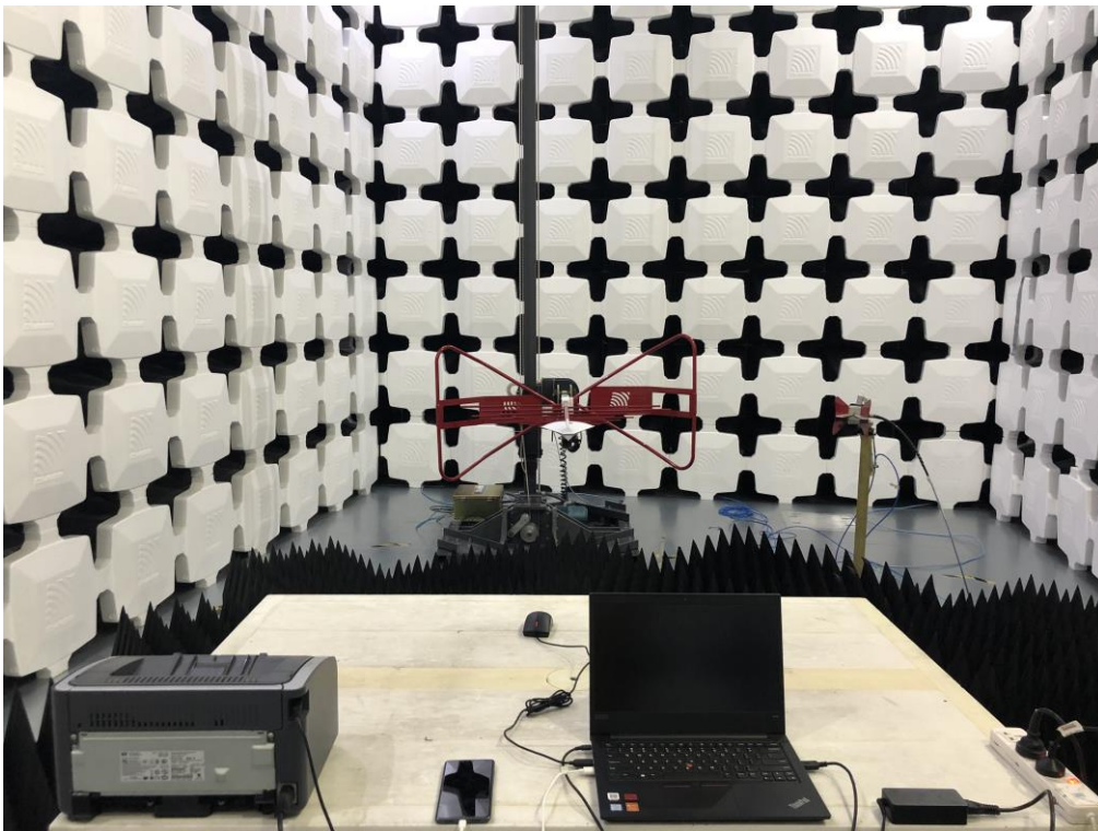
2. Radiated Emissions (Part 15B PC mode)(A1-18GHz)
