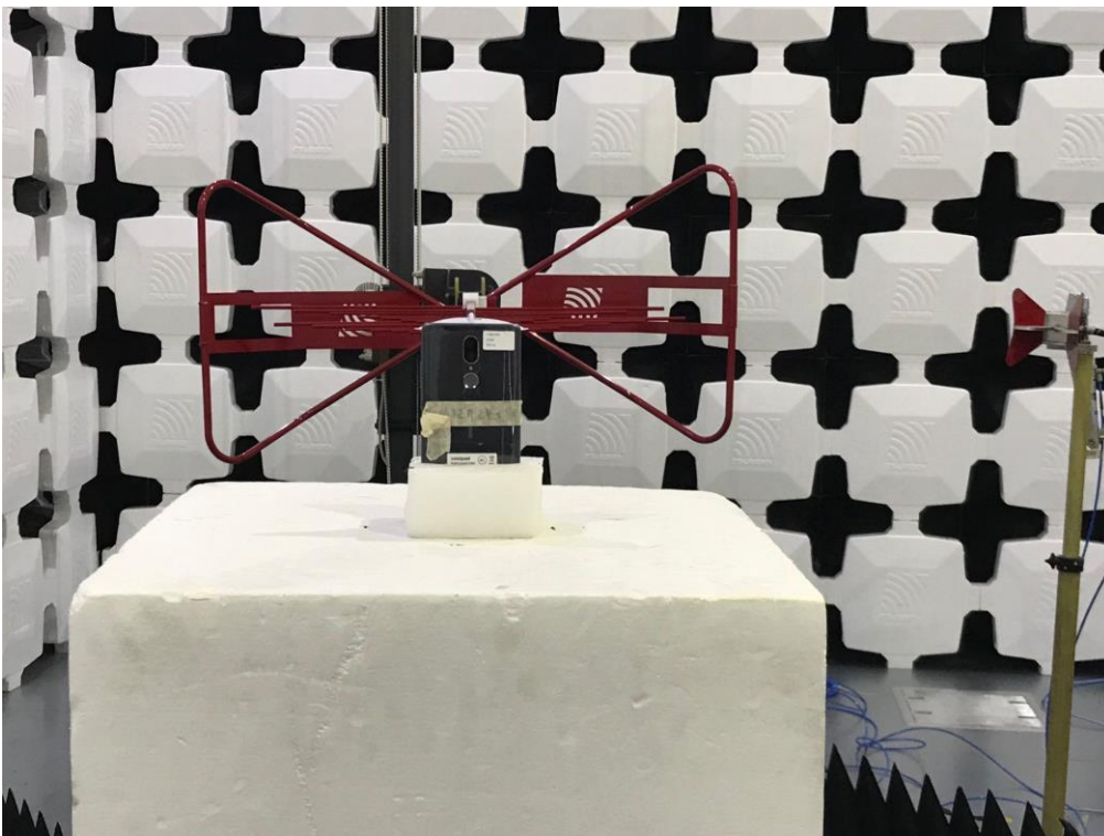
12. Radiated Emissions (Part 22/24) (30M-18GHz)
