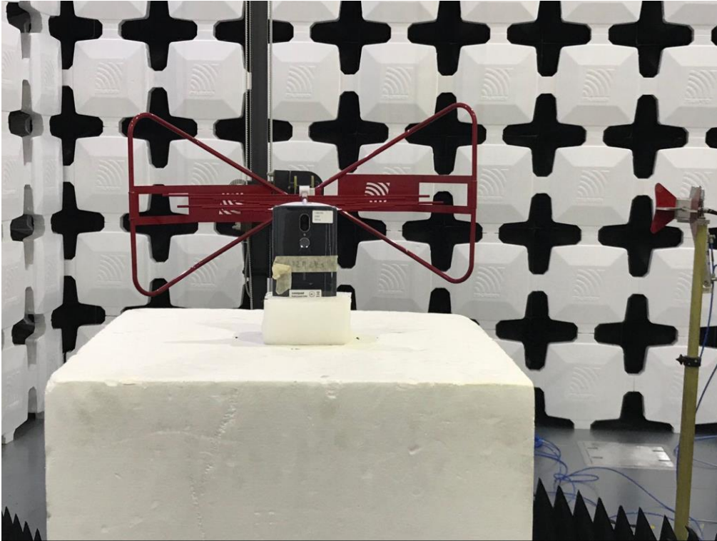
9. Radiated Emissions (Part 15C) (1-18GHz)
