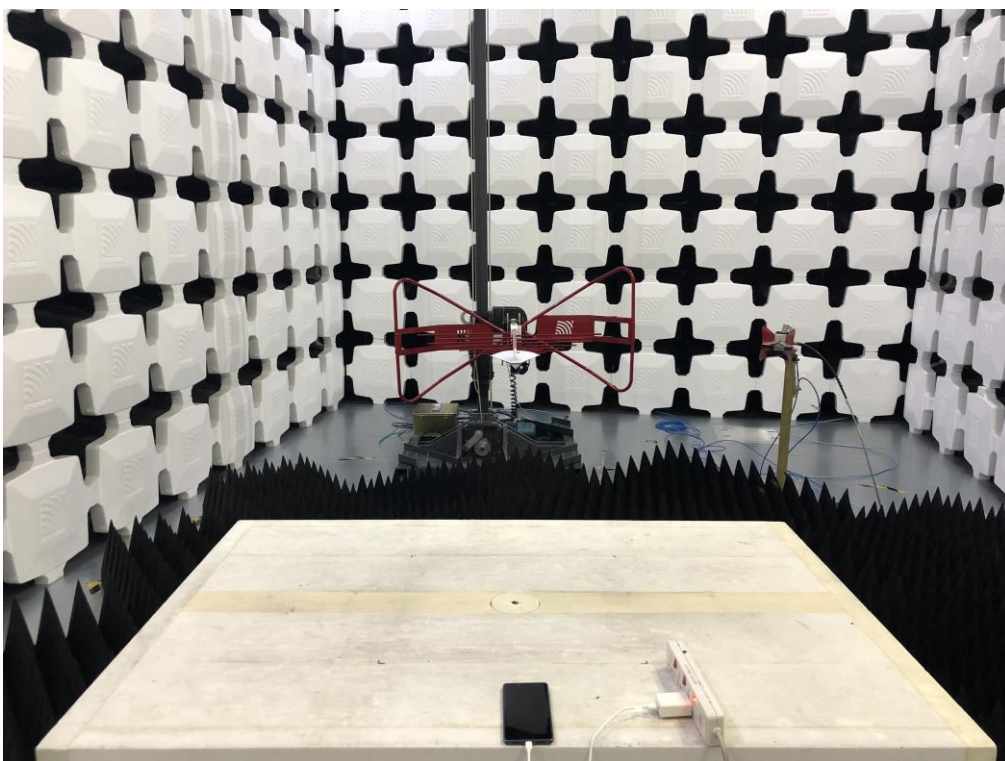
4. Radiated Emissions (Part 15B Charging mode) (1-18GHz)
