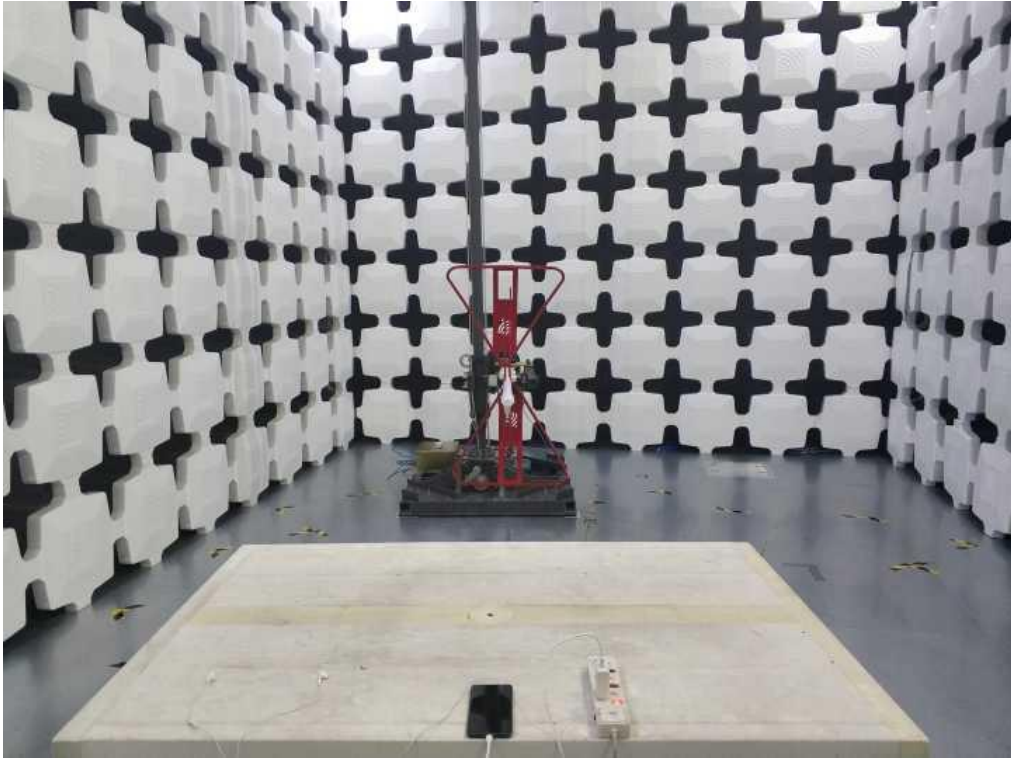
5. Radiated Emissions (Part 15B Charging mode-FM) (below 1GHz)
