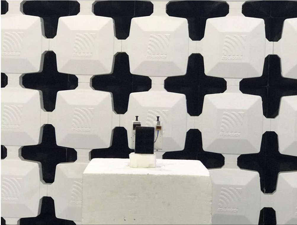
11. Radiated Emissions (Part 15C) (26.5-40GHz)
