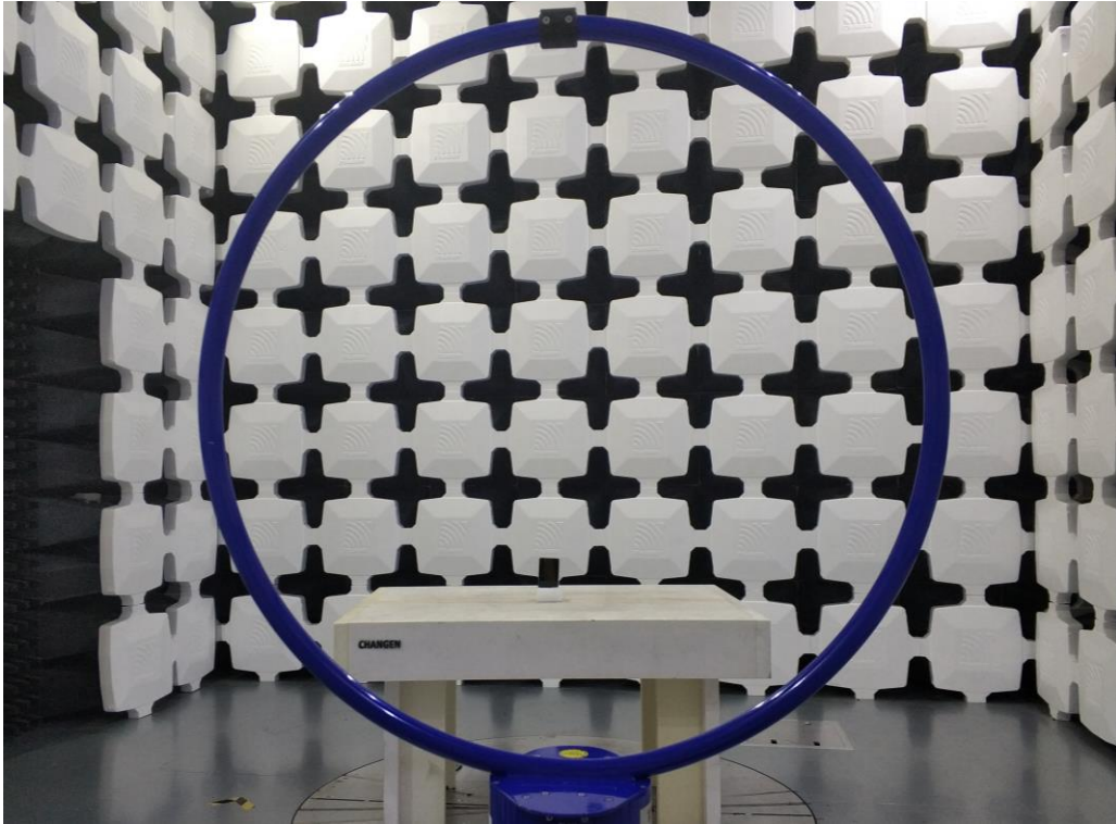
7. Radiated Emissions (Part 15C)( 9KHz-1GHz)
