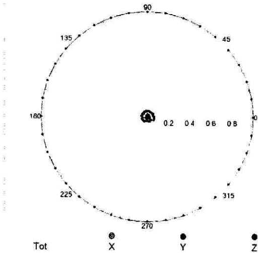
f=600 MHz, TEM, 90^\circ
