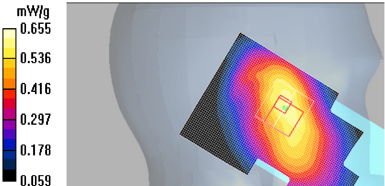
Fig.5 WCDMA 850 CH4132
