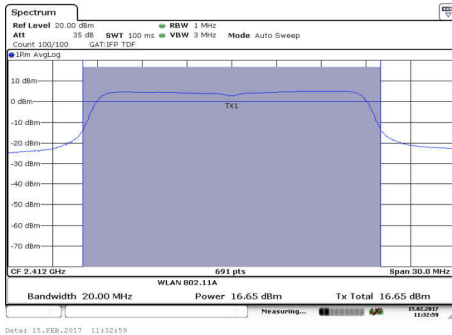
Fig.37 Maximum Average Output Power (802.11n-20MHz, Ch 1,MCS0)
