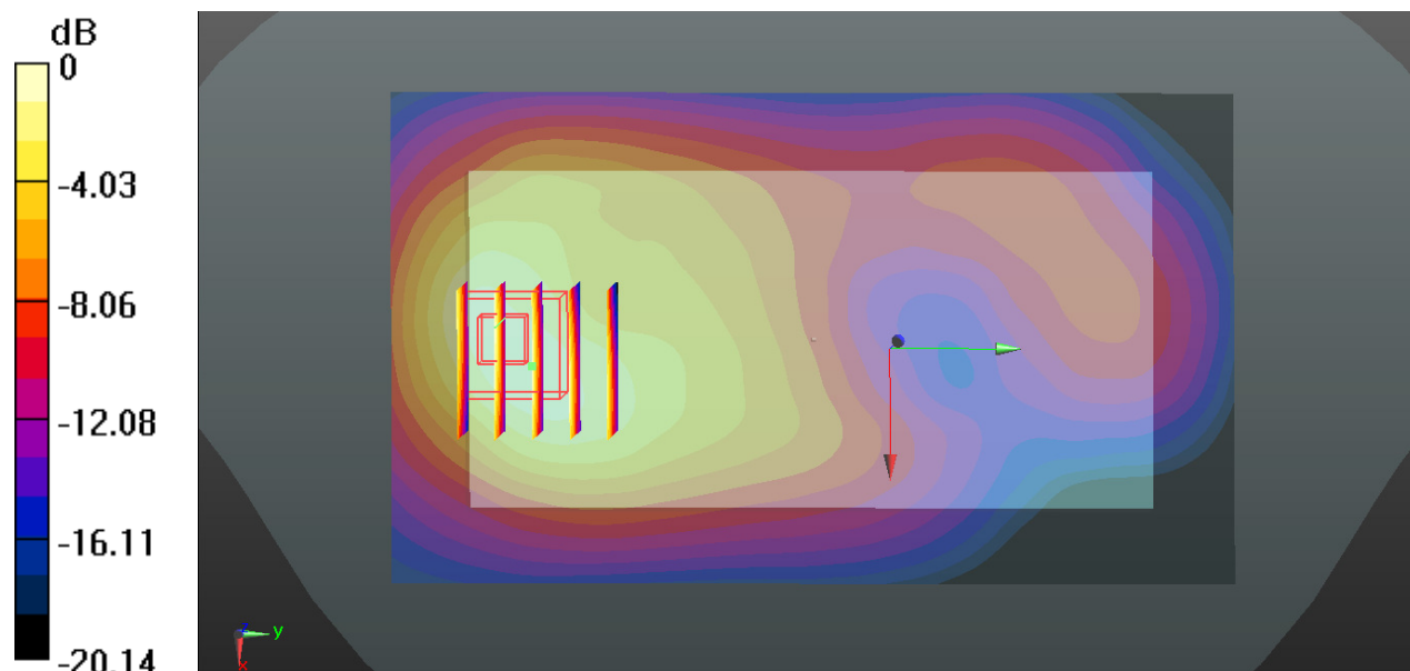
0 dB = 0.982 W/kg
