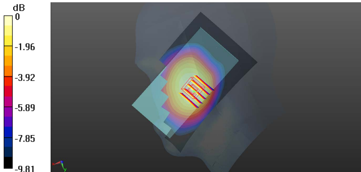
0 dB = 0.346 W/kg
