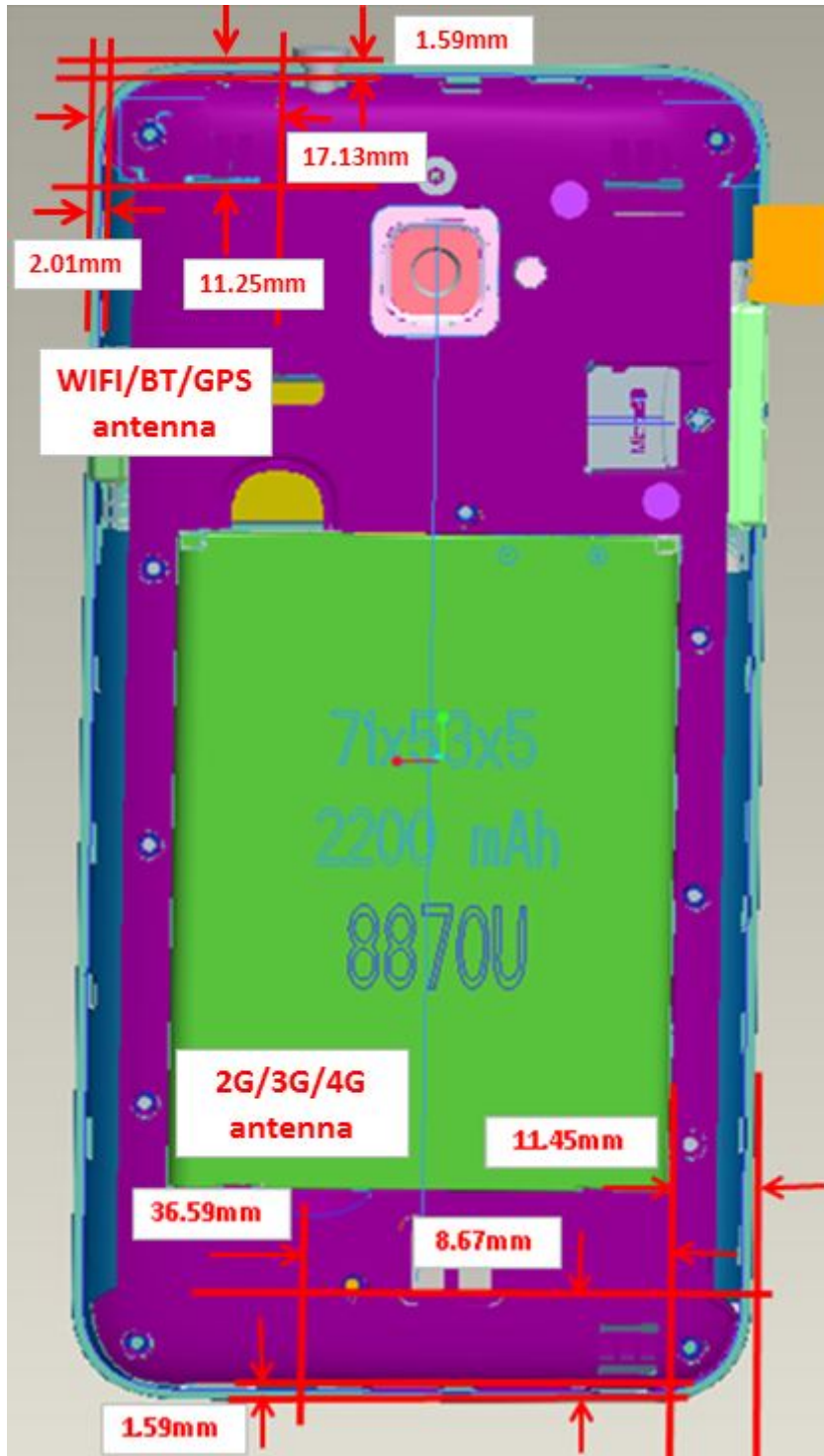
Antenna Location
