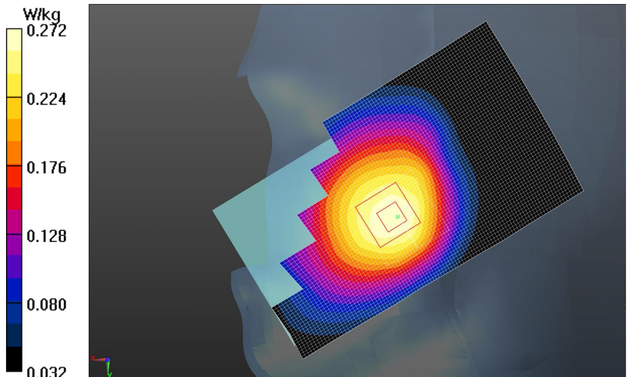
Fig.15 LTE Band 12
