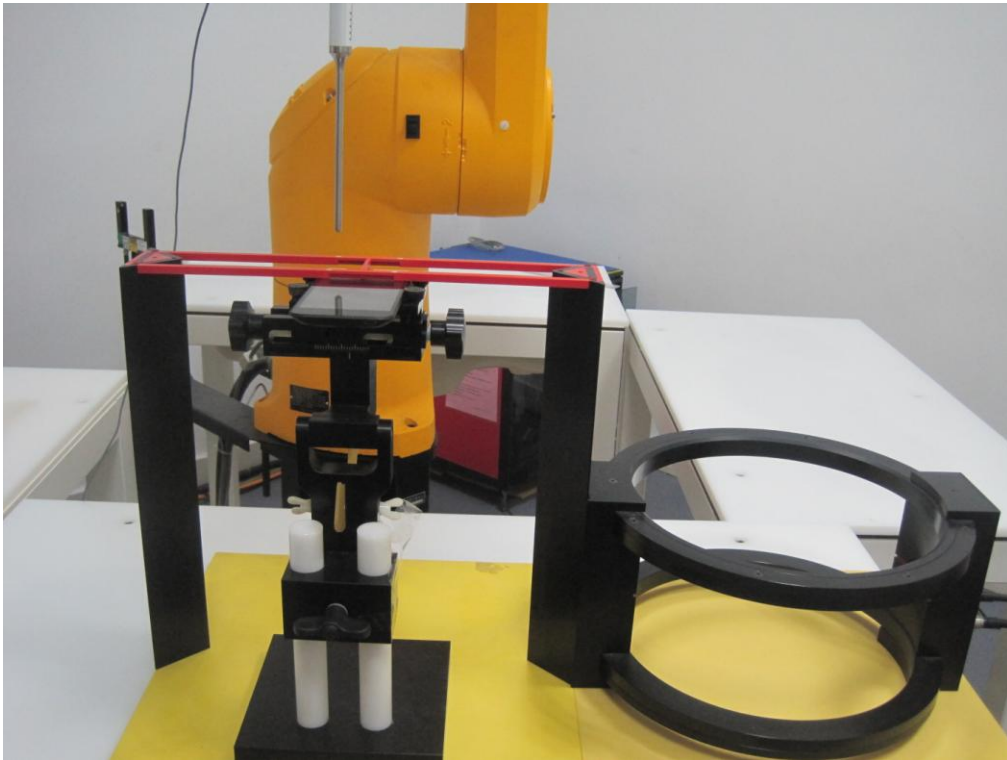
Picture 3: HAC T-coil set up photo
