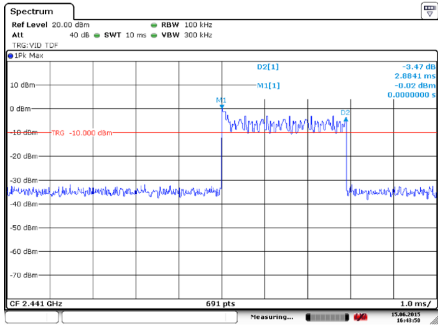
Fig. 91 Time of Occupancy(Dwell Time) (8DPSK, Ch39)
