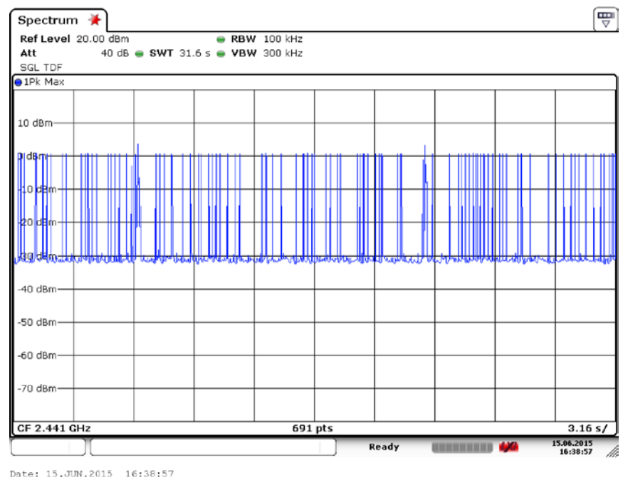
Fig. 88 Number of Transmissions (GFSK, Ch39)
