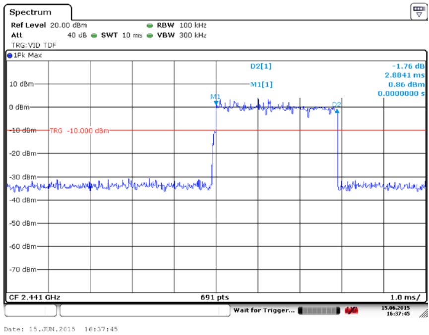
Fig. 87 Time of Occupancy(Dwell Time) (GFSK, Ch39)
