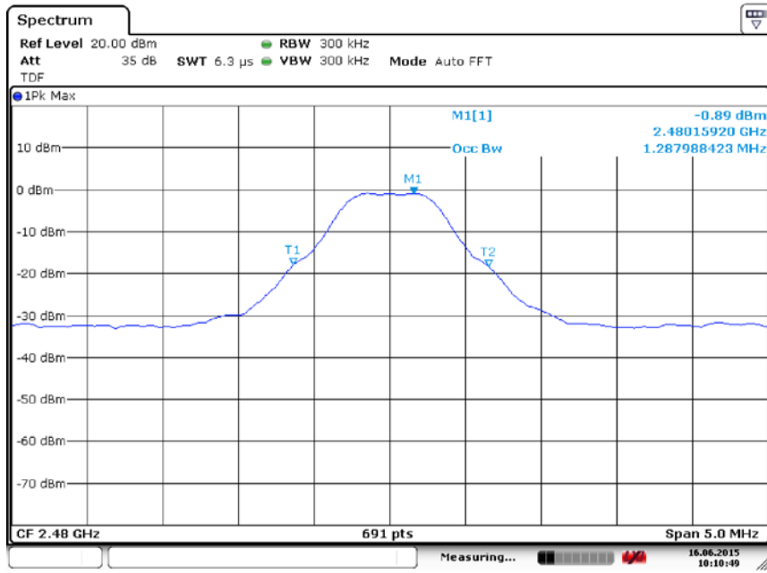
Fig.105 Occupied Bandwidth (GFSK, Ch 78)
