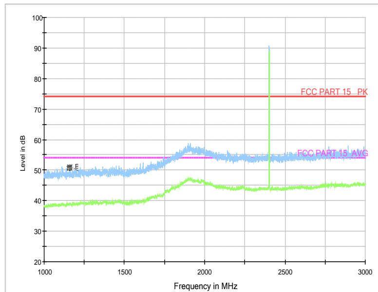
RE_BT_1G-3GHz
