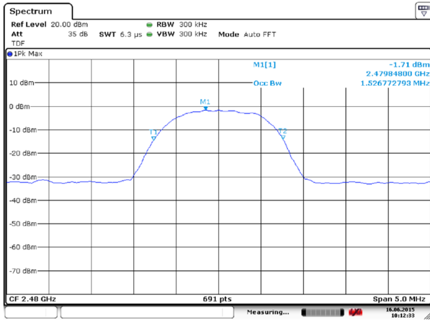
Fig.111 Occupied Bandwidth (8DPSK, Ch 78)
