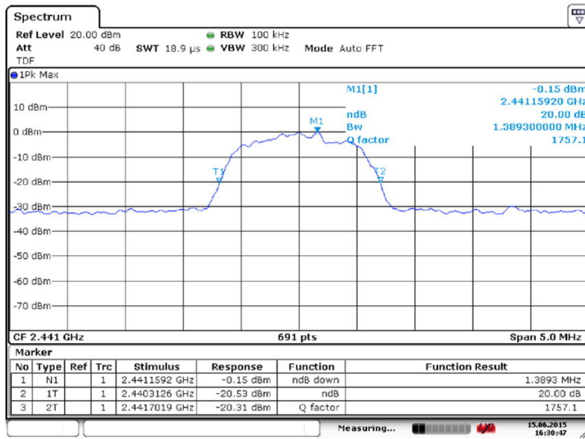
Fig. 85 Occupied 20dB Bandwidth (8DPSK, Ch 39)
