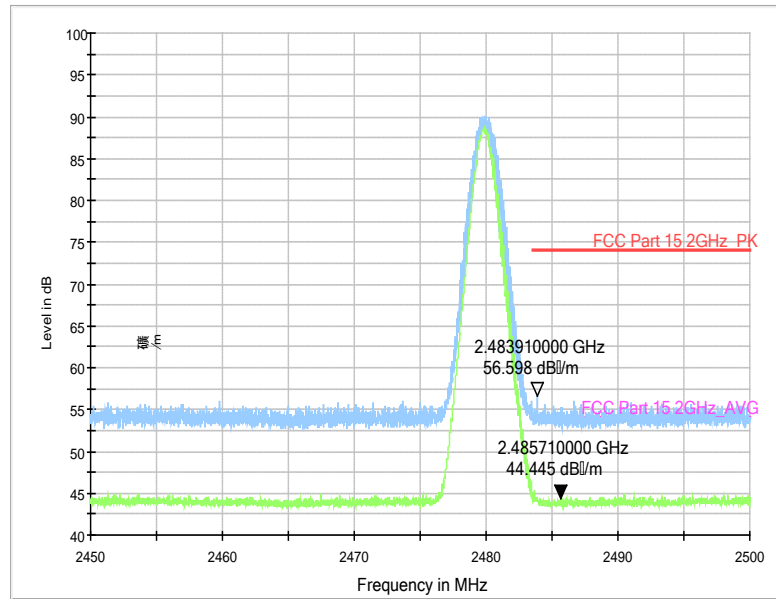
RE-BT-Power_2.45G-2.5GHz
