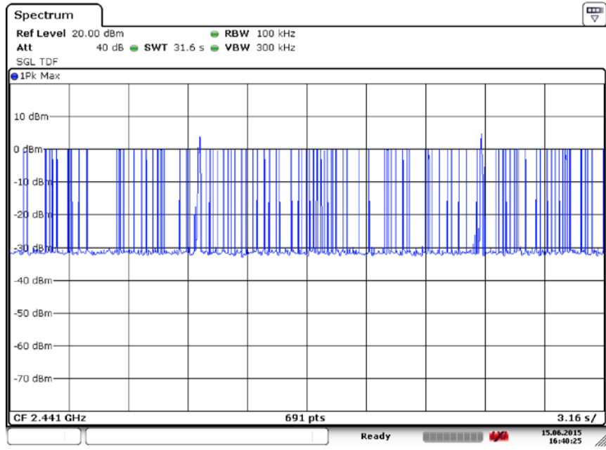
Fig. 90 Number of Transmissions ( \pi/4 DQPSK, Ch39)
