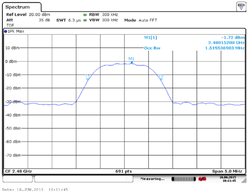
Fig.107 Occupied Bandwidth ( \pi/4 DQPSK, Ch 39)
