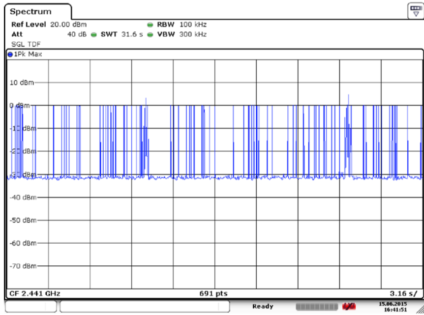
Fig. 92 Number of Transmissions (8DPSK, Ch39)
