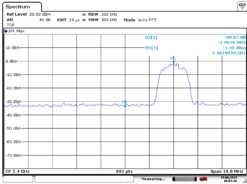
Fig. 20 Band Edges (8DPSK, Ch 0, Hopping OFF)
