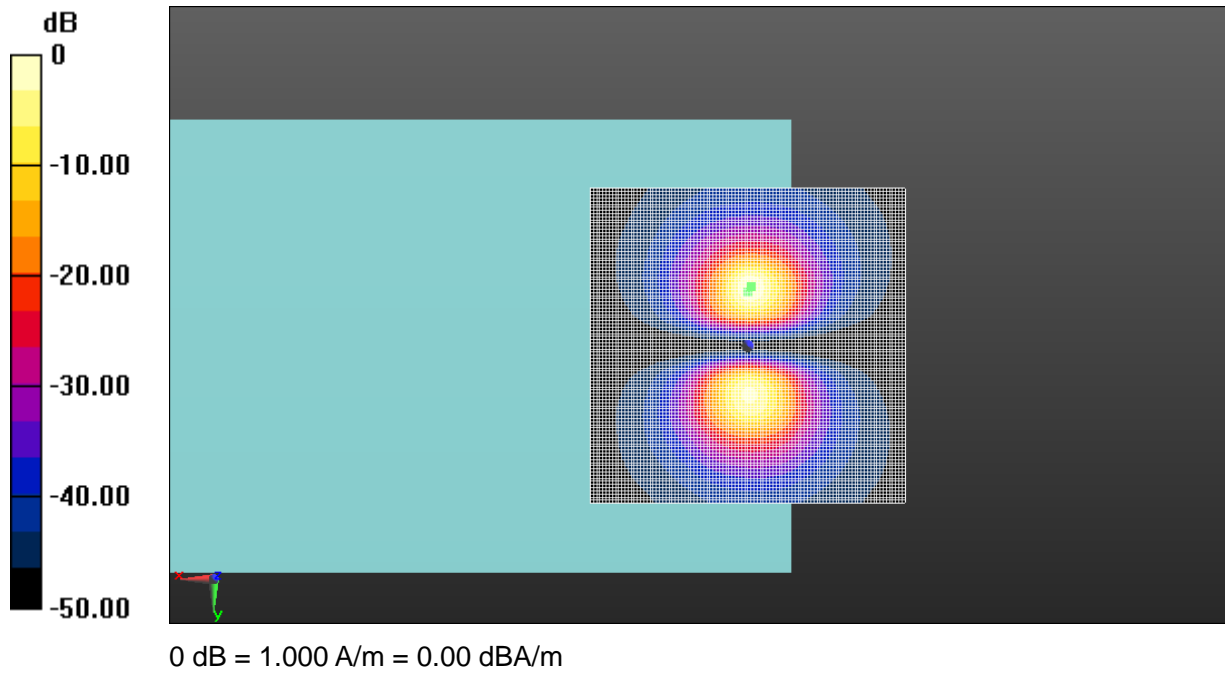
Fig A.14 T-Coil LTE-Band 4
