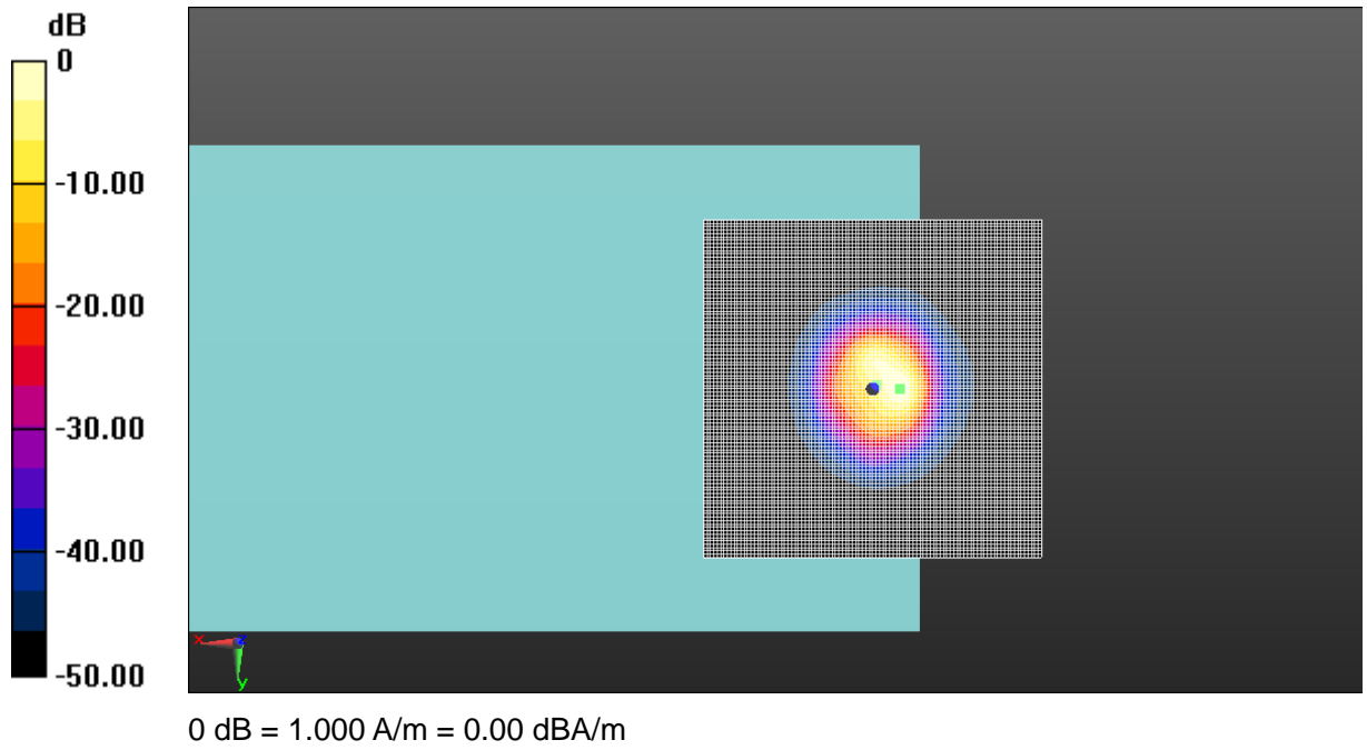
Fig A.9 T-Coil CDMA BC10
