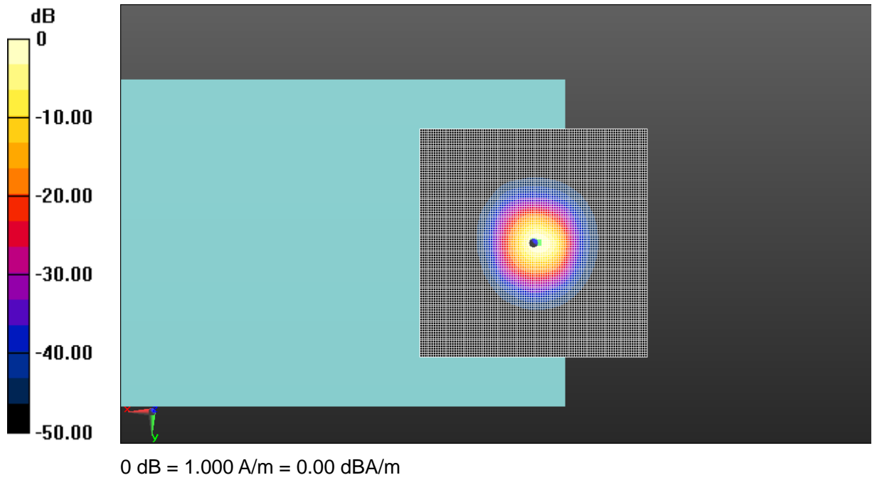
Fig A.15 T-Coil LTE-Band 5
