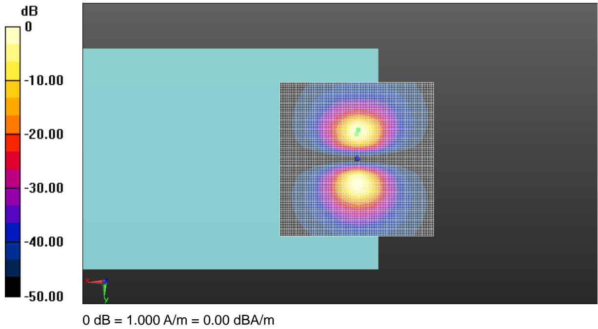
Fig A.18 T-Coil LTE-Band 13
