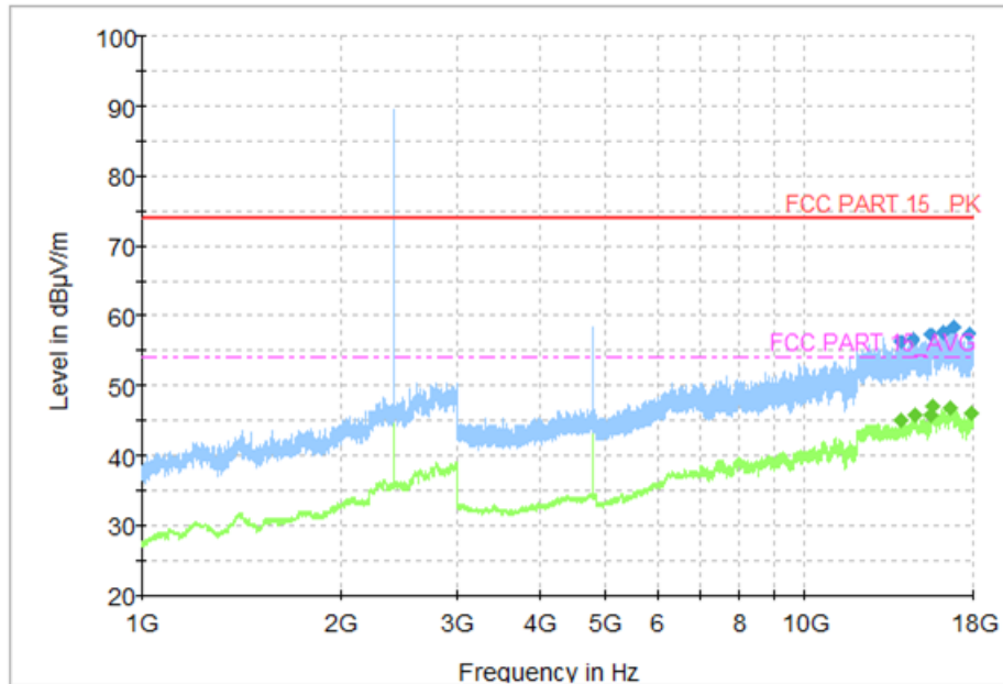
Fig.20 Radiated Spurious Emission (GFSK, Ch0, 1 GHz ~18 GHz)
