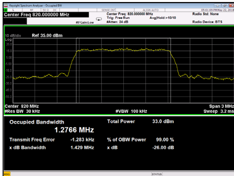
99% & 26dB Occupied Bandwidth Plot on Channel 560
