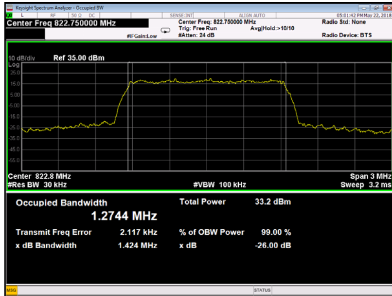
99% & 26dB Occupied Bandwidth Plot on Channel 670
