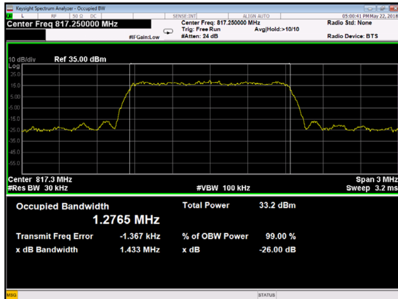
99% & 26dB Occupied Bandwidth Plot on Channel 450
