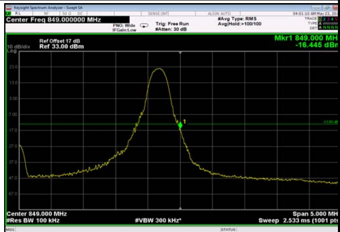
HighRange_FDD26_5MHz_846.5_fullRB _HighQ16
