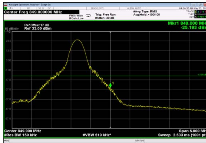
HighRange_FDD26_15MHz_841.5_fullIRB_HighQPSK
