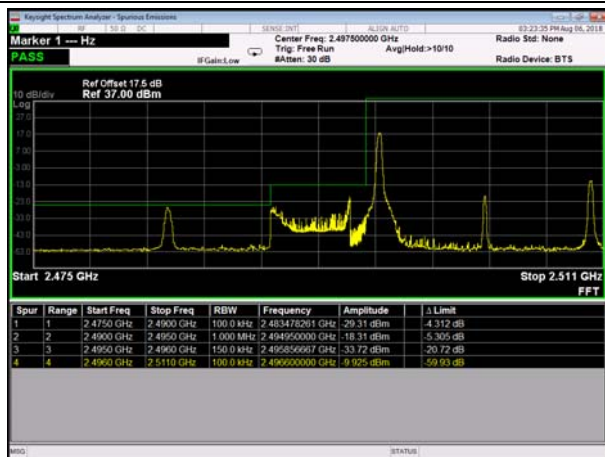
LowRange_TDD41_15MHz_2503.5_fullRB _LowQPSK
