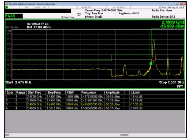
LowRange_TDD41_5MHz_2498.5_fullIRB_LowQ16
