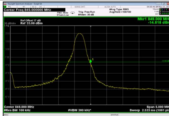
HighRange_FDD26_5MHz_846.5_fullRB _HighQPSK
