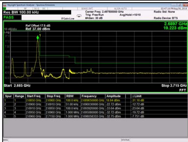
HighRange_TDD41_5MHz_2687.5_OneRB_high_QPSK
