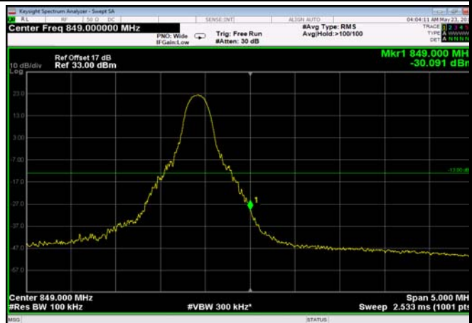
HighRange_FDD26_10MHz_844_OneRB _high_Q16
