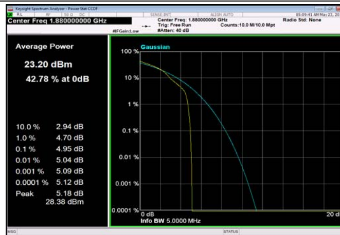
FDD02_5MHz_1880MHz_OneRB_high_Q16
