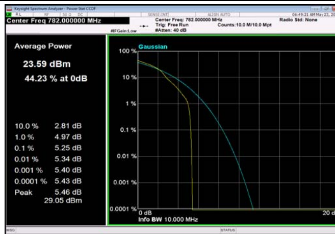
FDD13_5MHz_782MHz_OneRB_high_Q16
