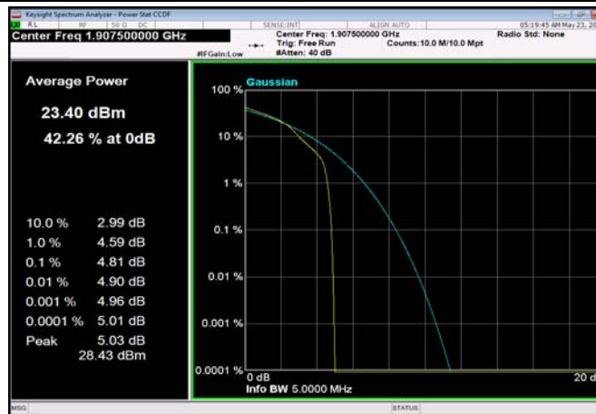
FDD02_5MHz_1907.5MHz_OneRB_high_Q16
