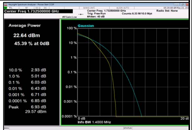
FDD04_1.4MHz_1732.5MHz_fullIRB_Q16
