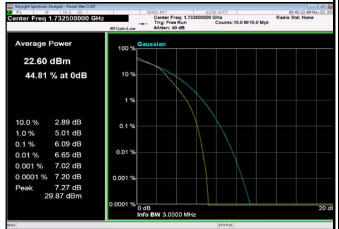
FDD04_5MHz_1732.5MHz_fullRB_Q16
