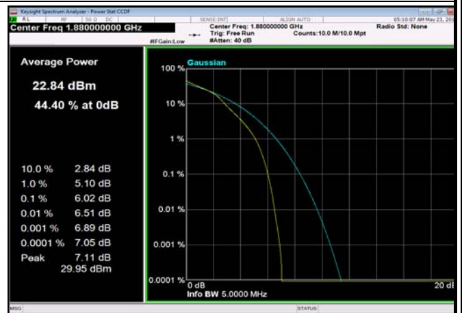
FDD02_5MHz_1880MHz_fullRB_Q16
