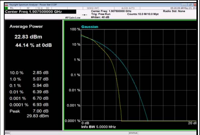
FDD02_5MHz_1907.5MHz_fullIRB_Q16
