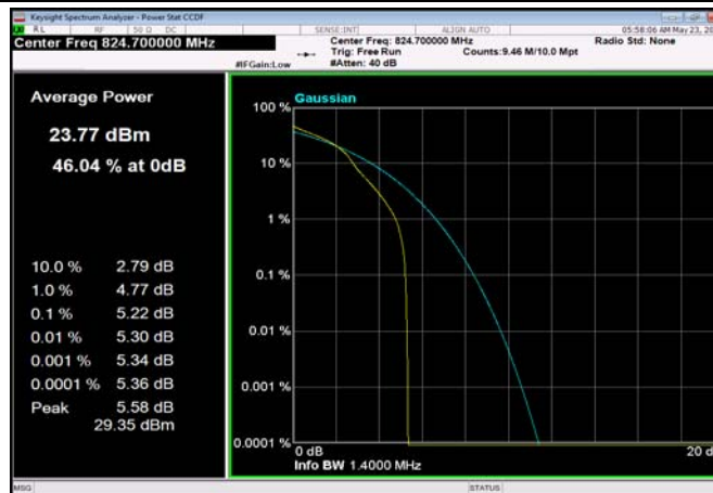
FDD05_1.4MHz_824.7MHz_OneRB_high_Q16
