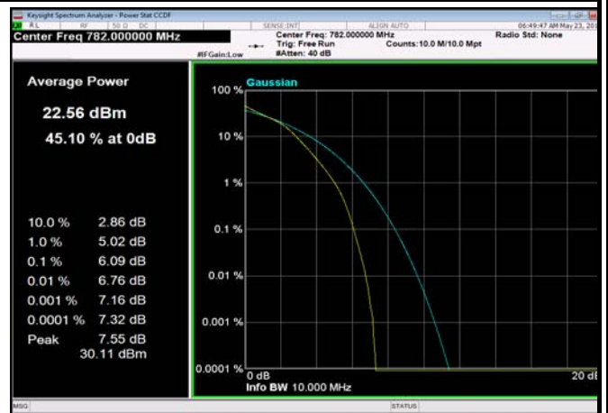
FDD13_5MHz_782MHz_fullRB_Q16
