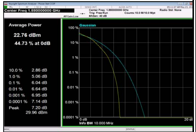
FDD02_15MHz_1880MHz_fullRB_Q16
