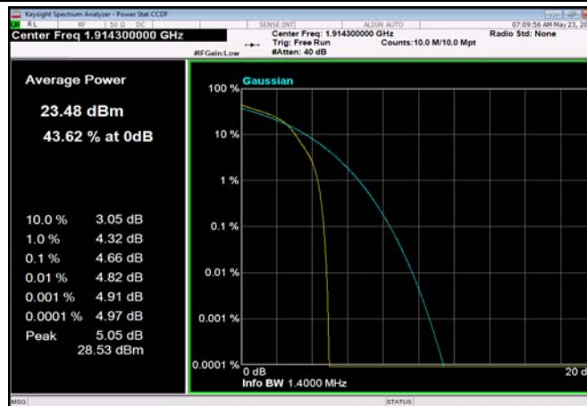
FDD25_1.4MHz_1914.3MHz_OneRB_high_Q16
