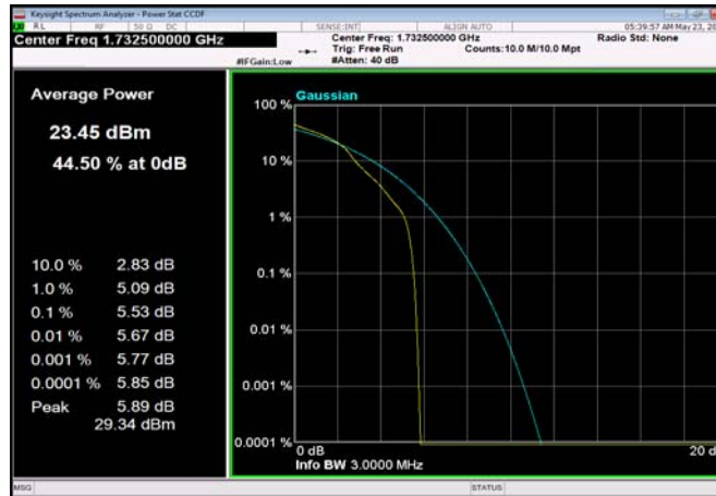
FDD04_5MHz_1732.5MHz_OneRB_high_Q16
