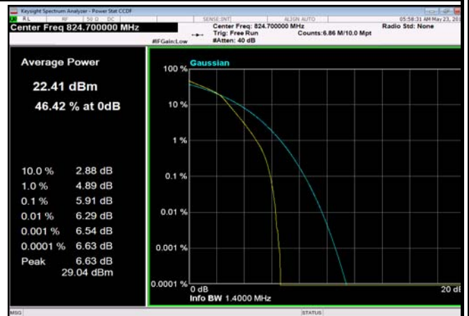
FDD05_1.4MHz_824.7MHz_fullIRB_Q16
