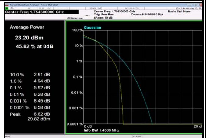
FDD04_1.4MHz_1754.3MHz_fullIRB_Q16
