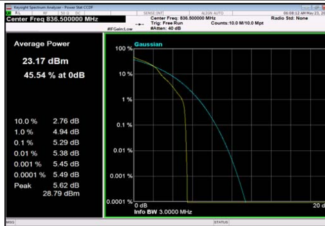
FDD05_5MHz_836.5MHz_OneRB_high_Q16
