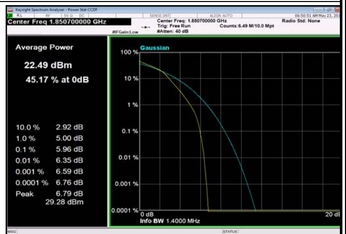
FDD25_1.4MHz_1850.7MHz_fullRB_Q16
