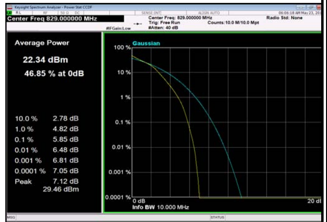
FDD05_10MHz_829MHz_fullRB_Q16
