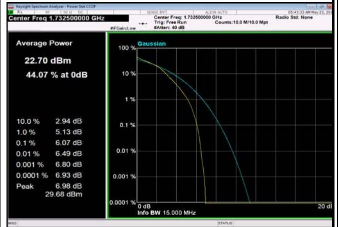
FDD04_20MHz_1732.5MHz_fullIRB_Q16
