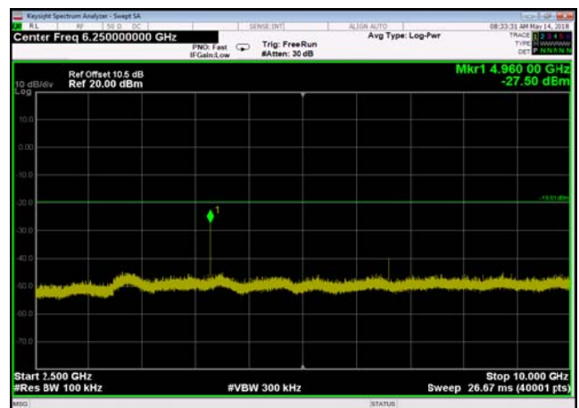
Transmitter Spurious Emission: 2480,25 000MHz~10000MHz
