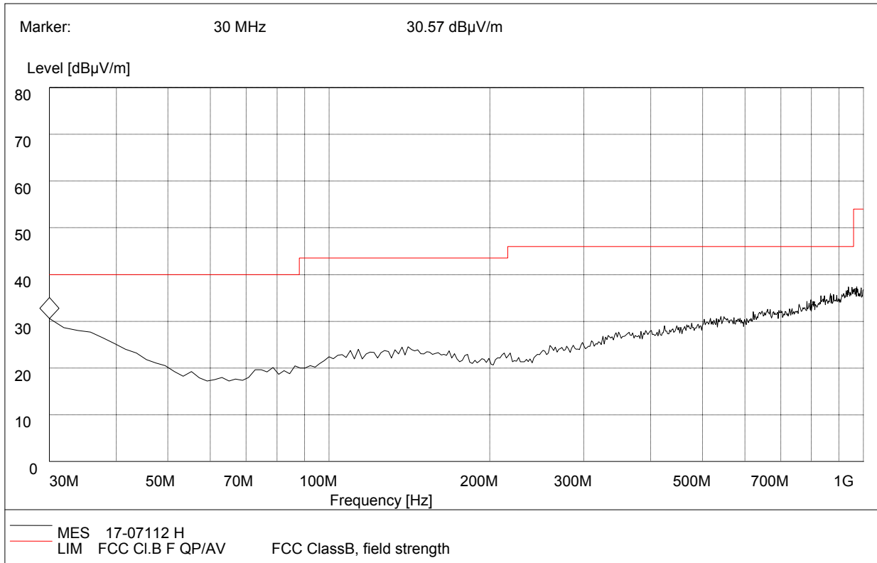
30MHz to 1GHz, Antenna Horizontal
