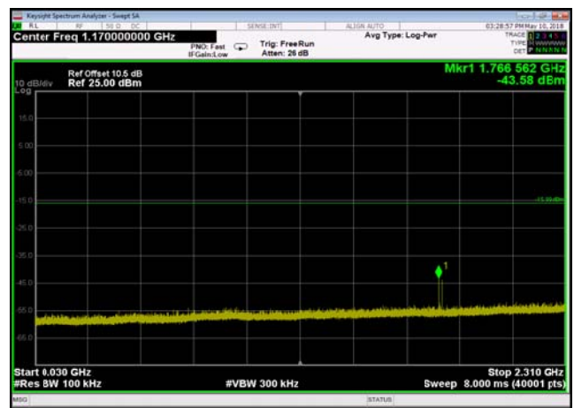
Conducted Emission: PI/4DQPSK,2480,2DH5,Reference Level
