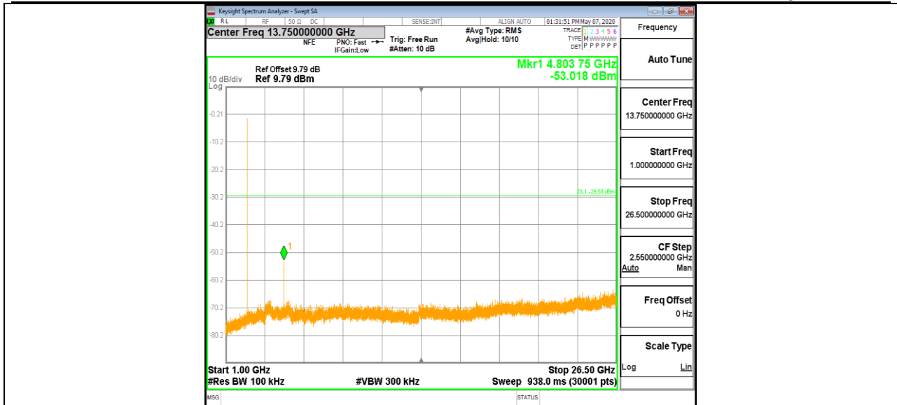
BLE_BT4.0_Ant1_2440_0~Reference
