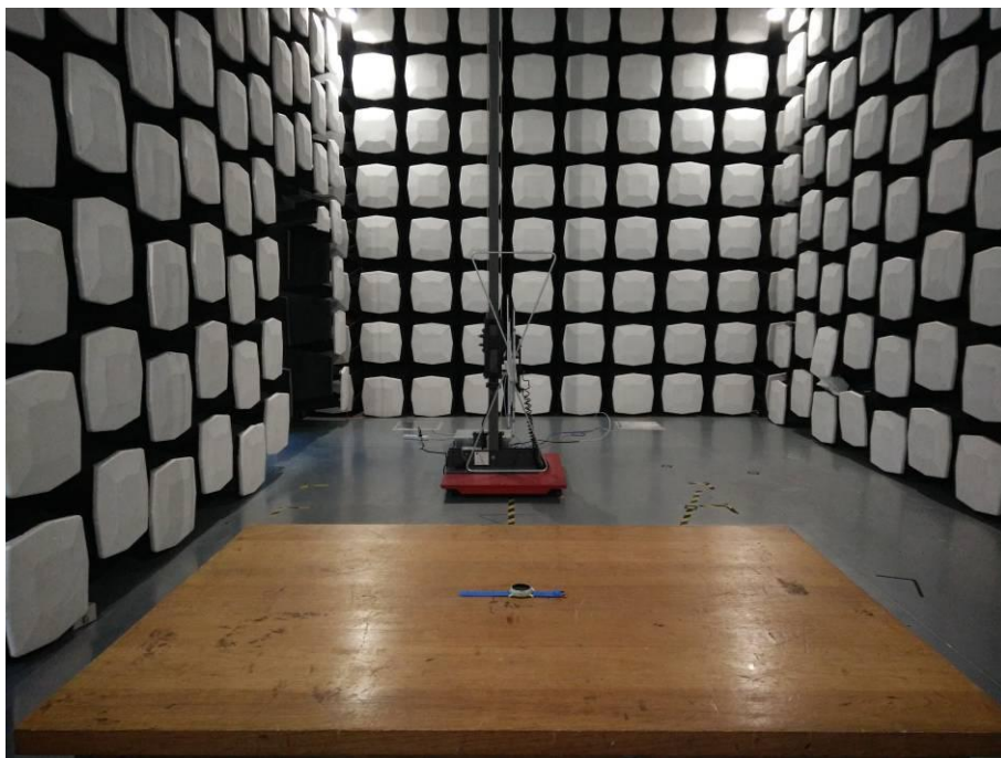
4. Radiated Emissions (Part 15C) 30M-1GHz)
