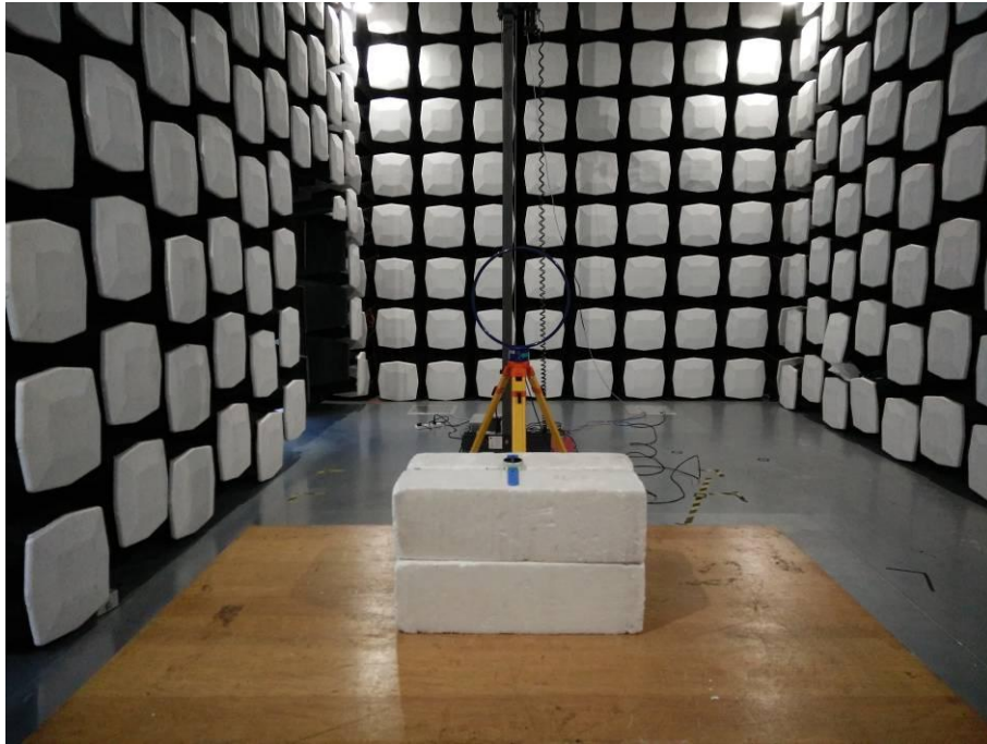
3. Radiated Emissions (Part 15C 9kHz-30M)
