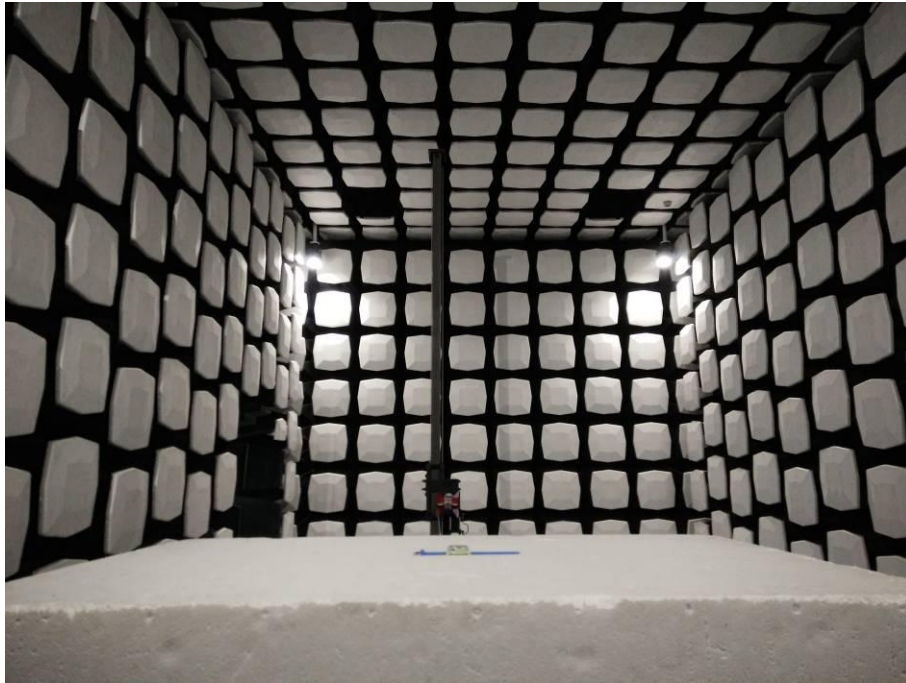
5. Radiated Emissions (Part 15C) (1-18GHz)
