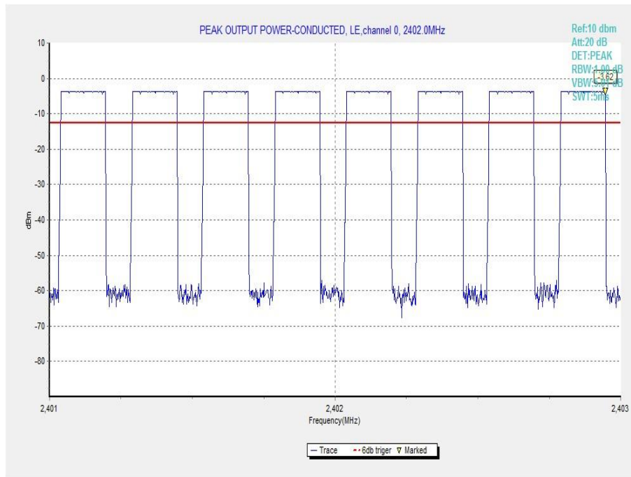
Fig.1 Maximum Peak Output Power(GFSK, Ch 0)
