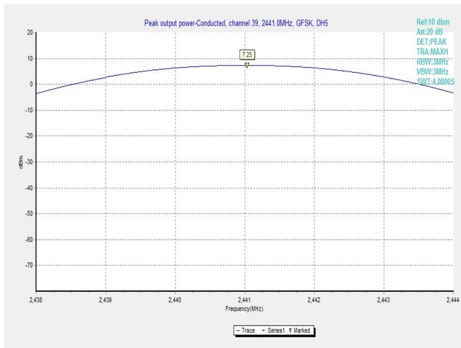
Fig. 2 Maximum Peak Output Power(GFSK, Ch 39)
