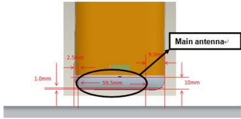
Antenna Location
