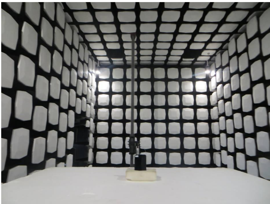
10. Radiated Emissions (Part 15C) (18-26.5GHz)
