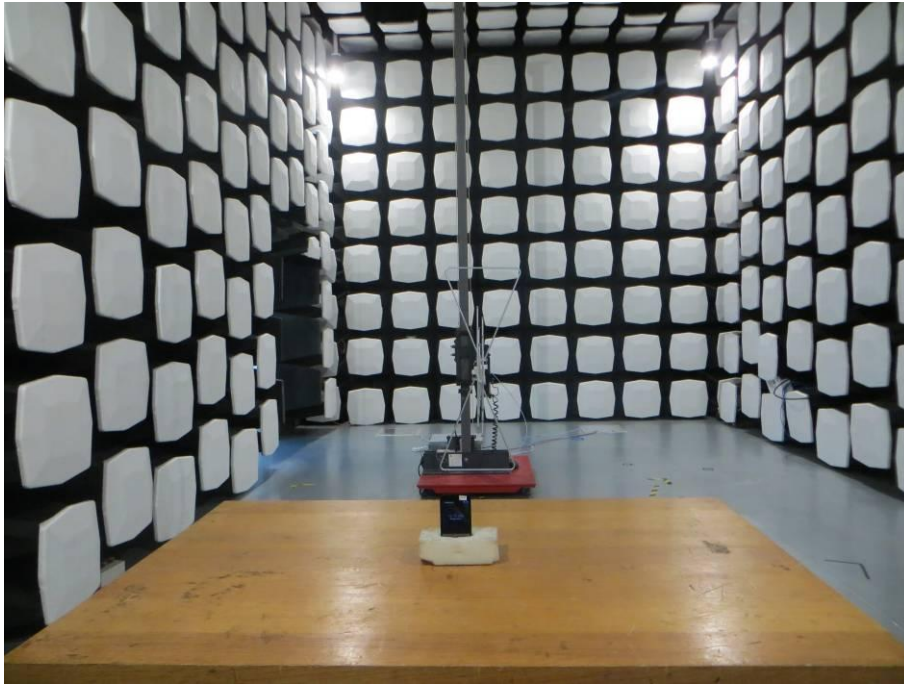
7. Radiated Emissions (Part 15C) 30M-1GHz)
