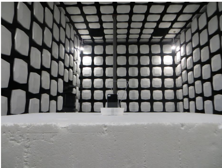
8. Radiated Emissions (Part 15C) (1-3GHz)
