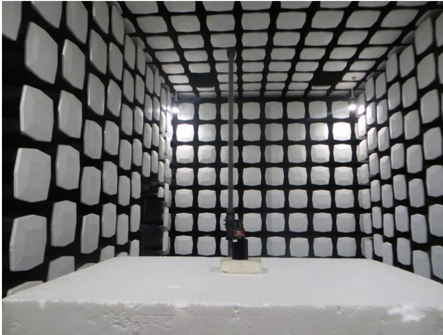
9. Radiated Emissions (Part 15C) (3-18GHz)
