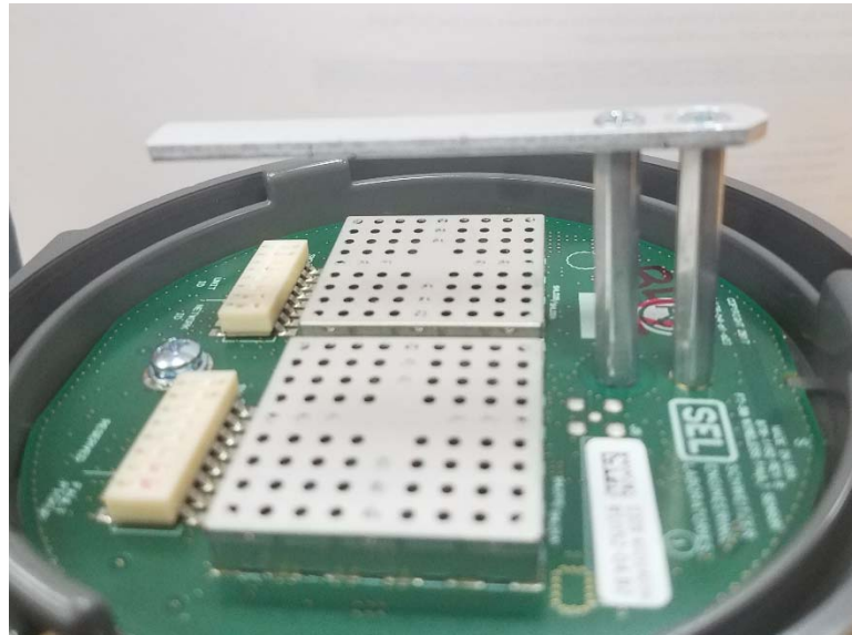
Figure 1 - SEL-WCS Inverted F Antenna
