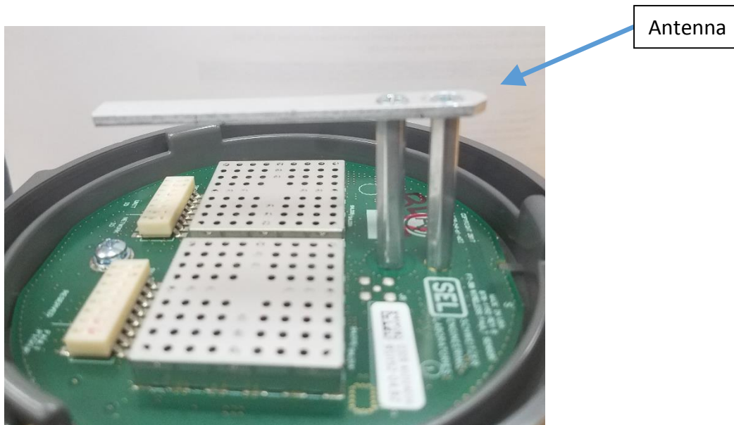
Figure 1 - SEL-FT50 Inverted F Antenna
